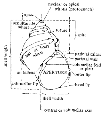
FIG. 2. Shell terminology.
