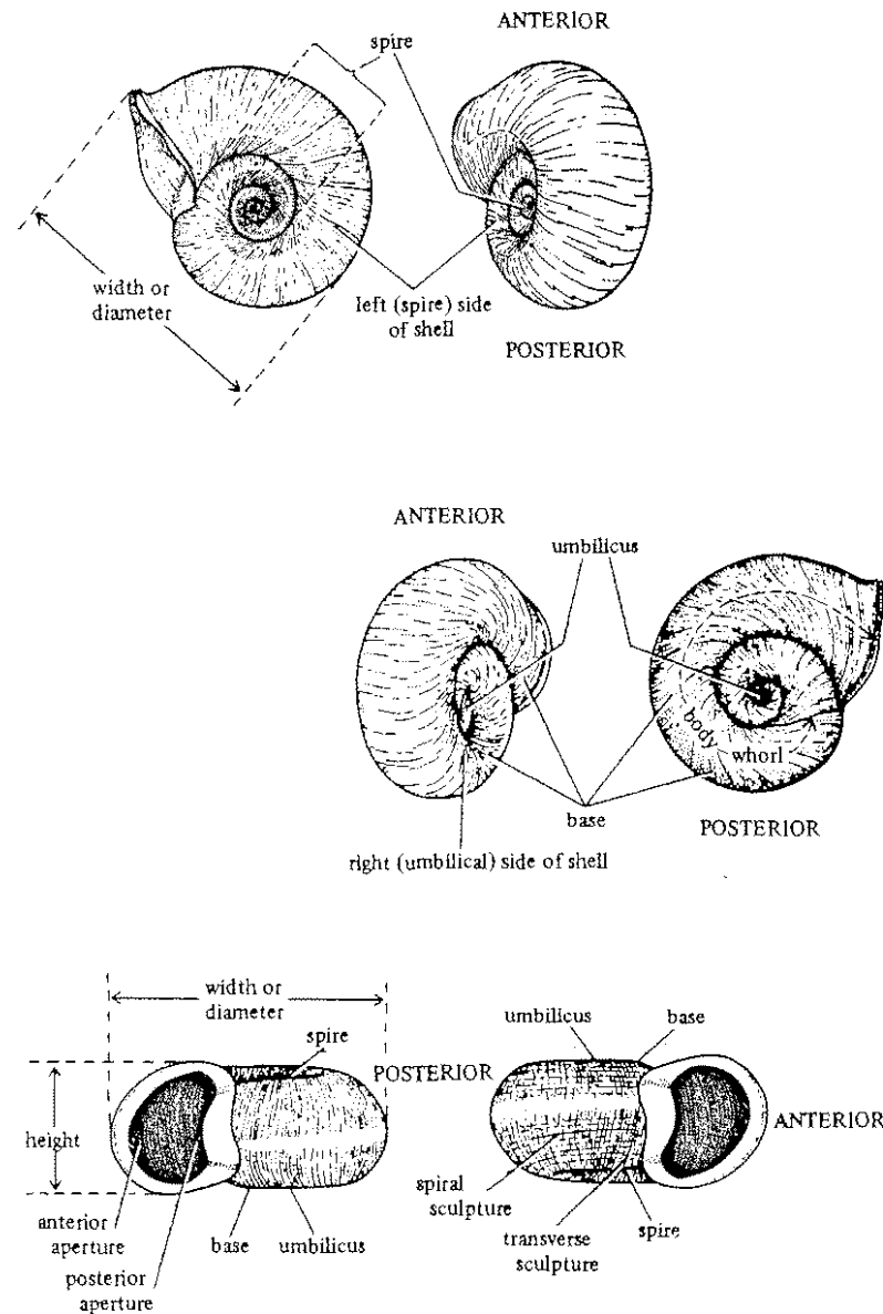
FIG. 704. Terminology of a planorbid shell.
