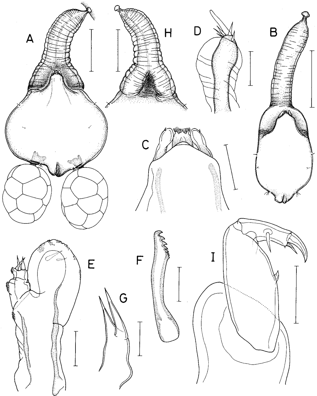
Fig. 16. Nectobrachia iceli , new species, female. A. Habitus, dorsal; B. Habitus of juvenile, dorsal; C. Cephalothorax (= head), dorsal; D. Antennule; E. Antenna; G. Maxillule; H. Maxilla (= arm), posterior; I. Maxilliped. Scales: 0.5 mm in A, B, H; 0.1 mm in C; 0.01 mm in D-G; 0.05 mm in I.
