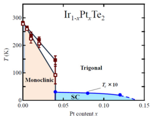
Figure 63. Phase diagram of \text{Ir}_{1-x}\text{Pt}_x\text{Te}_2 determined using single-crystal samples. Closed and open squares respectively represent the trigonal–monoclinic transition temperature T_s upon heating and cooling (the ‘monoclinic’ phase corresponds to the triclinic phase in figure 62, representing the simplified symmetry). Closed circles represent the T_c and SC represents the bulk superconducting region. The hatched area represents a temperature range of broad hysteresis in resistivity. Reprinted with permission from [63]. Copyright 2012 by the Physical Society of Japan.
