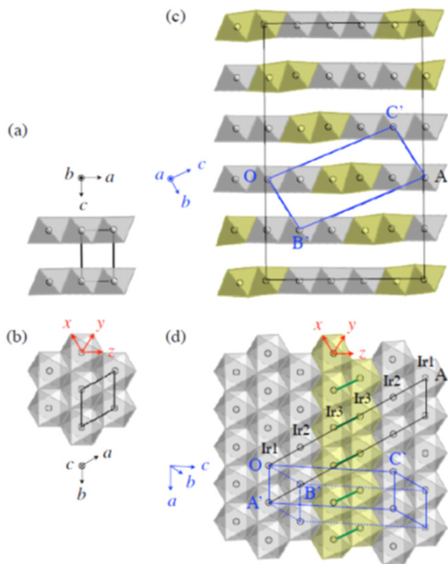
Figure 62. (a), (b) The crystal structure of \text{IrTe}_2 at 300 K. Black lines represent the unit cell of the trigonal lattice. (c), (d) The crystal structure of \text{IrTe}_2 at 20 K. Blue lines represent the unit cell of the triclinic lattice. Black lines represent the 5a \times b \times 5c supercell ( a , b , and c are the high-temperature trigonal-cell parameters). Reprinted with permission from [374]. Copyright 2014 by the Physical Society of Japan.
