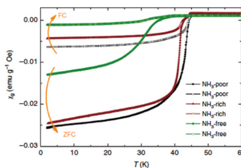
Figure 25. The magnetization curves of three Na/ \text{NH}_3 intercalated FeSe measured with the zero-field-cooling (ZFC) and field-cooling (FC) modes at H = 10 Oe. Reprinted with permission from Macmillan Publishers Ltd: [29], Copyright 2014.
