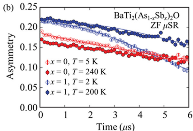
Figure 31. (a) Selected area electron diffraction patterns taken along the [001] axis for \text{BaTi}_2\text{Sb}_2\text{O} at 300 K and 14 K. (b) Asymmetry versus time spectra from zero-field muon spin relaxation measurements on \text{BaTi}_2\text{As}_2\text{O} and \text{BaTi}_2\text{Sb}_2\text{O} . Reprinted with permission from [277]. Copyright 2013 by the American Chemical Society.
