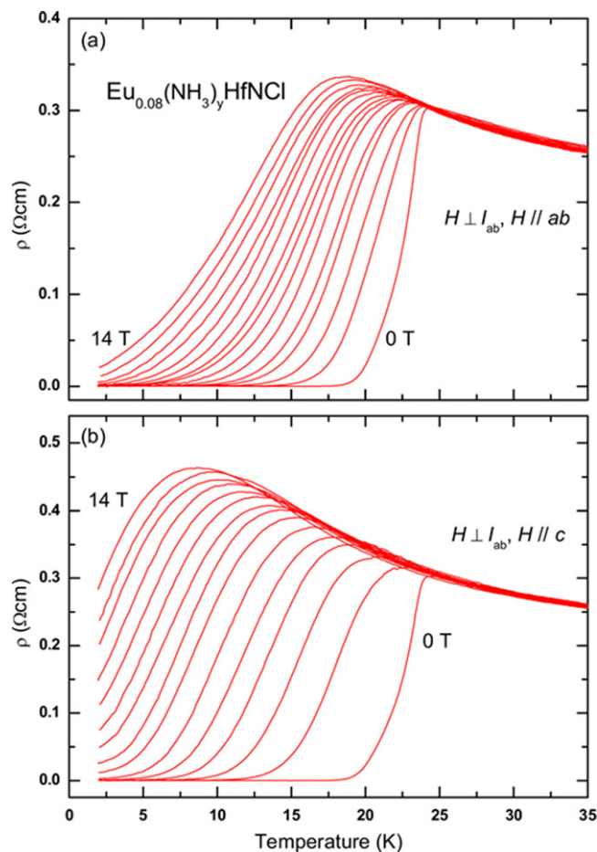
Figure 37. Temperature dependences of the resistivity of \text{Eu}_{0.08}(\text{NH}_3)_y\text{HfNCl} in various magnetic fields for (a) H \parallel ab ( H \perp I_{ab} ) and (b) H \parallel c ( H \perp I_{ab} ). The applied magnetic field was increased from 0 to 14 T with an interval of 1 T. Reprinted with permission from [60]. Copyright 2013 by IOP Publishing.
