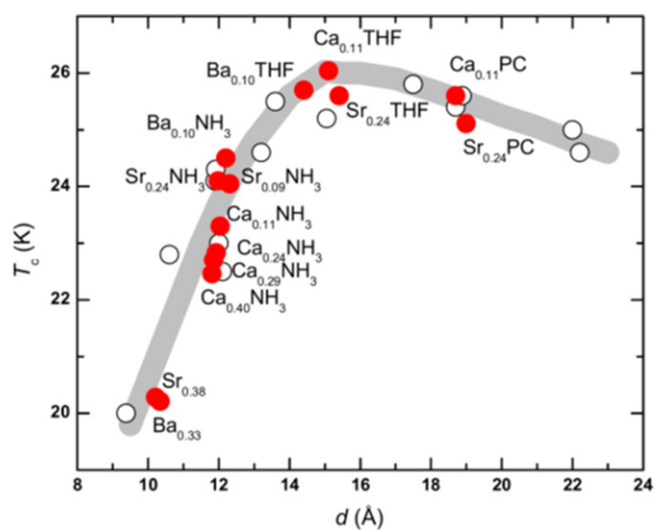
Figure 38. T_c dependence on the basal spacing d of AE_x(\text{Solv})_y\text{HfNCl} (●), and from alkali metal and rare earth metal intercalated compounds (○). Reprinted with permission from [59]. Copyright 2013 by IOP Publishing.
