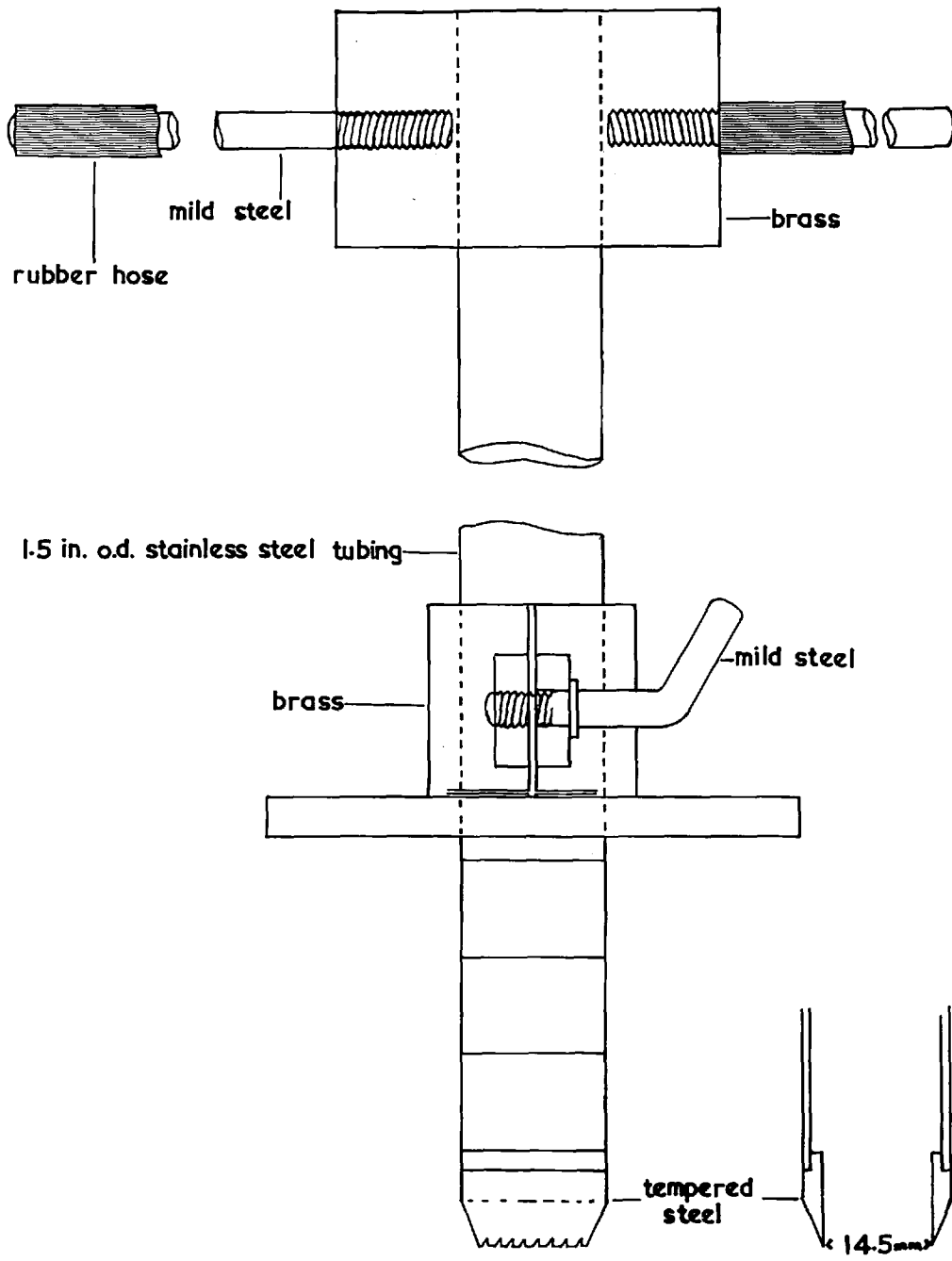
Fig. 1. Construction of the soil sampler.
