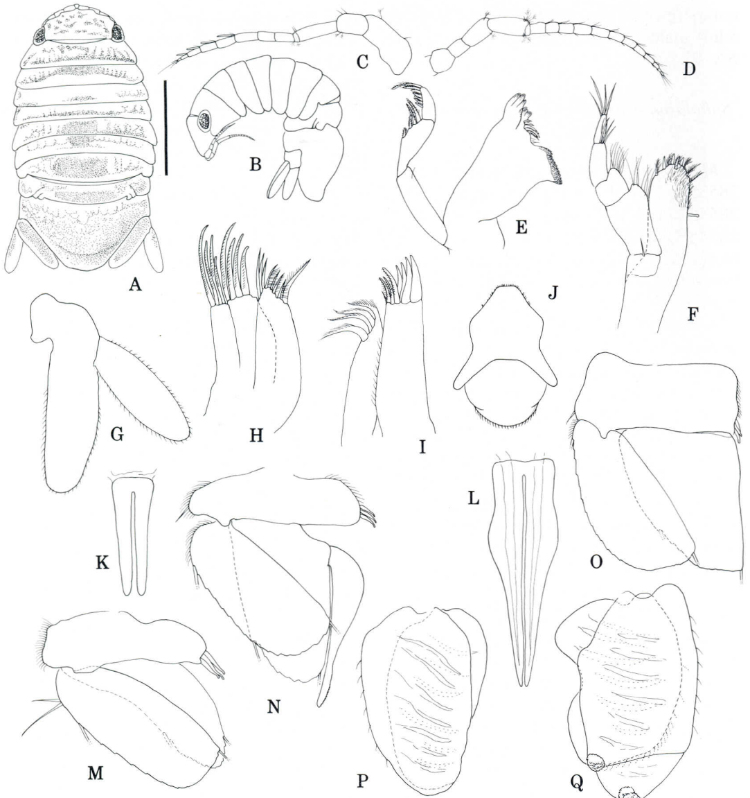
Fig. 7. Sphaeromopsis sanctaluciae , new species: A, adult male, habitus. Scale = 1 mm; B, lateral view; C, antennule; D, antenna; E, mandible; F, maxilliped; G, uropodal rami; H, maxilla 2; I, maxilla 1; J, ventral cephalon; K, penes of sub-adult male; L, penes of adult male; M, pleopod 1; N, pleopod 2; O, pleopod 3; P, pleopod 4; Q, pleopod 5.
