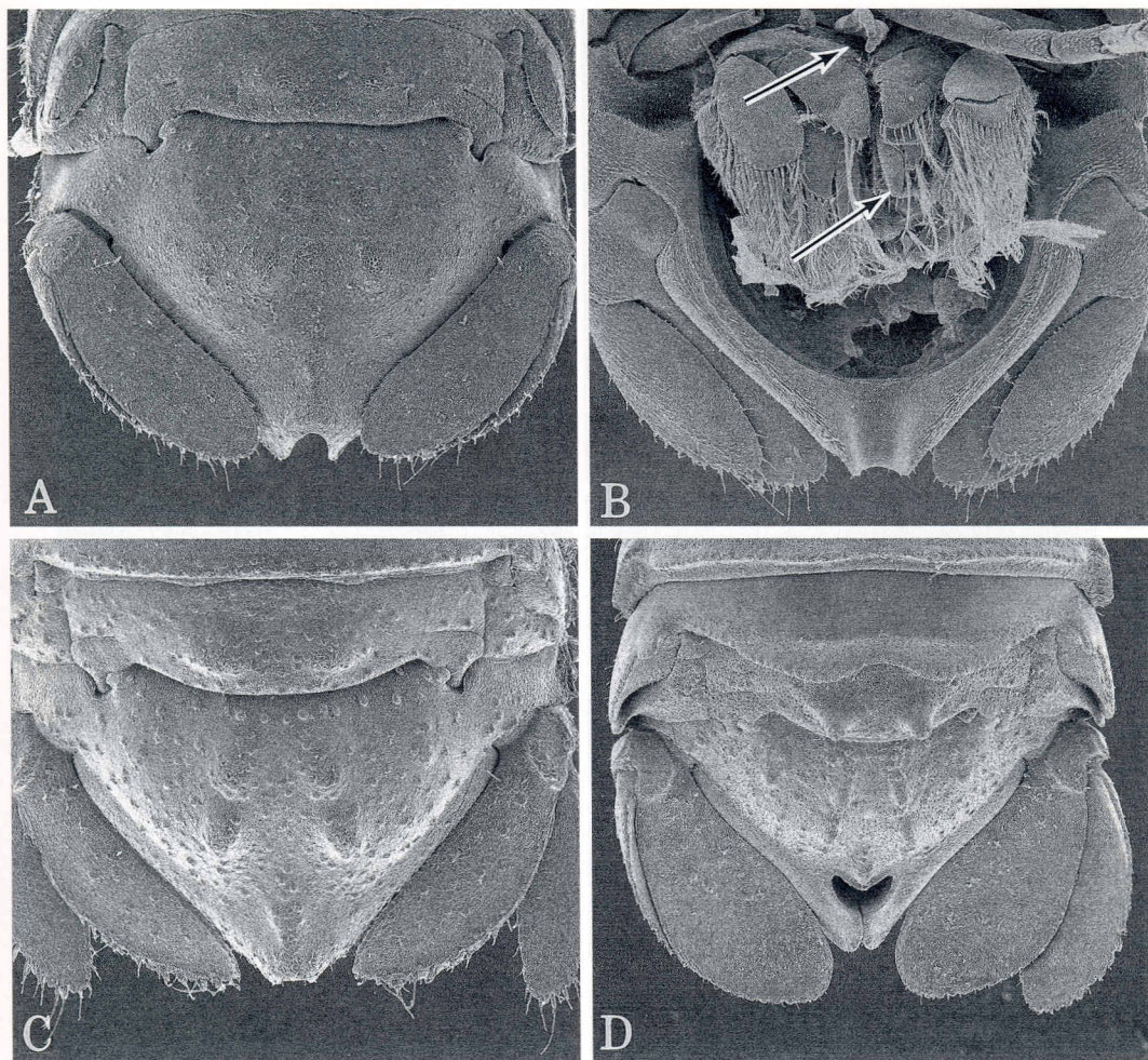
Fig. 5. Paradella diana : A, sub-adult male, dorsal pleotelson; B, sub-adult male, ventral pleotelson, arrows indicating immature penes and appendix masculina; C, ovigerous female, dorsal pleotelson; D, mature male, dorsal pleotelson.
