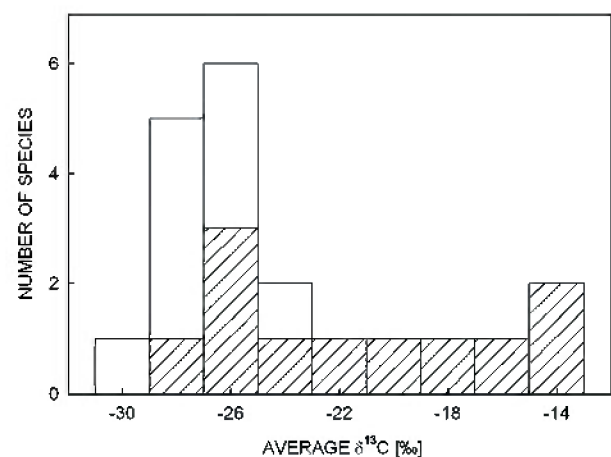
Fig. 1. Frequency of leaf \delta^{13}\text{C} for Mexican species of Clusia with presence (diagonal) or absence (open) of CAM. The presence of CAM was based on carbon stable isotopes values and on previously published data. Each bar represents a 2 ‰ range of \delta^{13}\text{C} .
