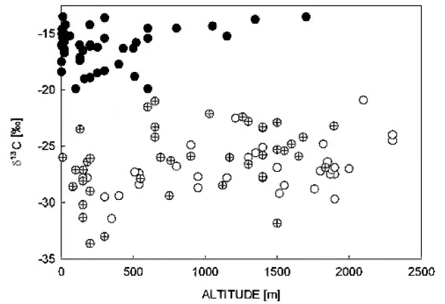
Fig. 3. Relationship between leaf \delta^{13}\text{C} values and altitude for Mexican species of Clusia that exhibited strong CAM (closed circles), those known to perform CAM (crossed circles), and those in which CAM has not been detected (open circles).
