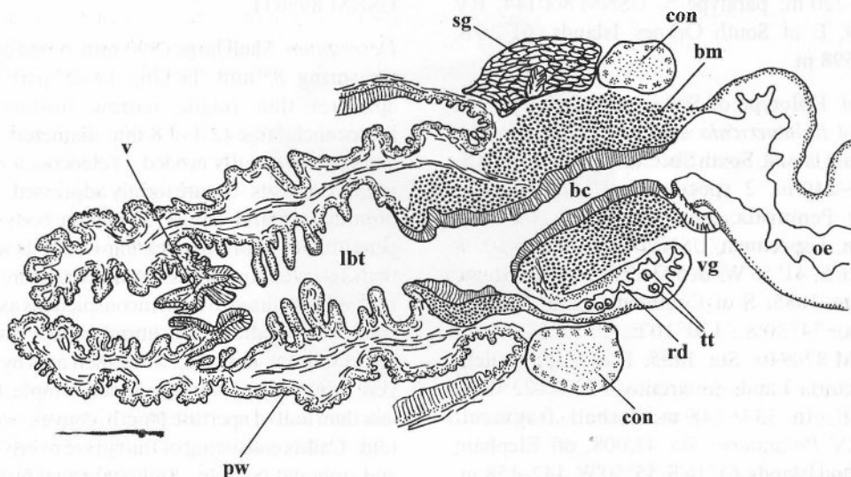
Fig. 2. Semi-diagrammatic longitudinal section through the proboscis. Salivary ducts and loops of the venom gland are not shown. A radular tooth is shown below the proboscis tip at the same scale. Abbreviations: bc = buccal cavity, bm = buccal mass, con = circumoesophageal nerve ring, lbt = lumen of the buccal tube, oe = oesophagus, pw = proboscis wall, rd = radular caecum, sg = salivary gland, tt = radular teeth, v = valvule, vg = venom gland.
