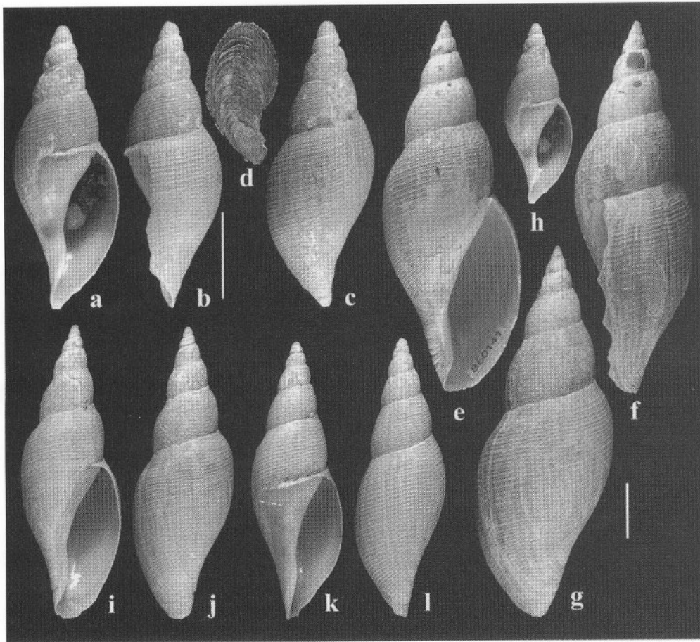
Fig. 1. Belaturricula gaini (Lamy, 1910). a–d. Holotype of Sipho gaini Lamy, 1910. (d. operculum). Scale bar = 1 cm. h. Holotype of Sipho gaini at the same scale as other specimens in figure. e–g. Holotype of Belaturricula antarctica Dell, 1990, USNM 860141, i–j. USNM 901688, k–l. USNM 901689 (anatomy examined). Scale bar = 1 cm.
