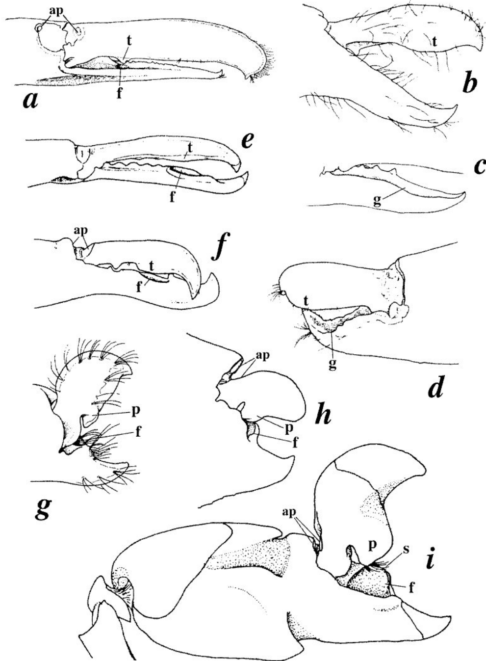
FIG. 5. Tooth-cavity systems on chela fingers of various Alpheidae: (a) Thylamea camelus ; (b,c) Vexillipar repandum ; (d) Bannereus anomalus ; (e) Nennalpheus sibogae ; (f) Amphibetaeus jousseaunei , major claw; (g) Synalpheus doriae , major claw; (h) Racilius compressus , major claw; (i) Alpheus edwardsii , major claw. Abbreviations: ap, adhesive plaques; f, fossa (more or less deep cavity); g, groove; p, plunger; s, stamen-shaped sensillae; t, tooth (in a,f) or thickening/bulge (b–e). (a–f,h,i) Adapted from Anker (2001b); (g) adapted from Bruce (1988b).
