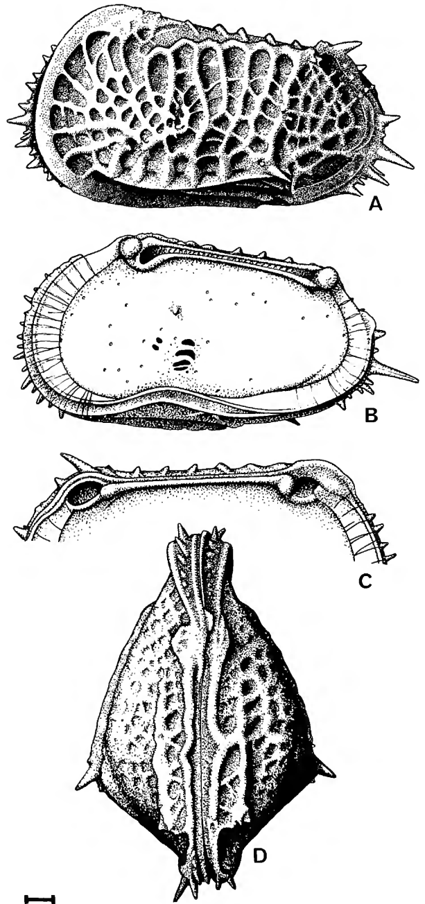
FIGURE 22.—Drawings of the carapace Poseidonamicus major , new species, from Mozambique Channel (IIOE 363B) showing (A) the general aspect of the surface sculpture, (B) the fused duplicature and thaeocytherid muscle scar pattern, (C) the holamphidont hinge elements, and (D) a dorsal view of a whole specimen. Scale = 100 microns.
