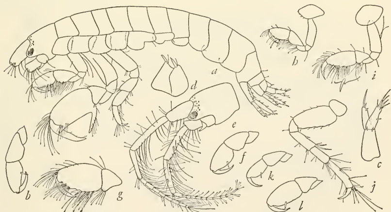
FIGURE 30.— Eurystheus digitatus Schellenberg, male, 3.7 mm., Reish sta. E-40: a , lateral view; b , gnathopod 1; c , uropod 3; d , telson; ?female, 5 mm., Reish sta. E-93: e , head; f, g , gnathopods 1, 2; female, 3 mm., Abbott sta. 15-C-2: h, i , gnathopods 1, 2; j , pereopod 5; female, 3.4 mm., Reish sta. E-93: k, l , gnathopods 1, 2.
