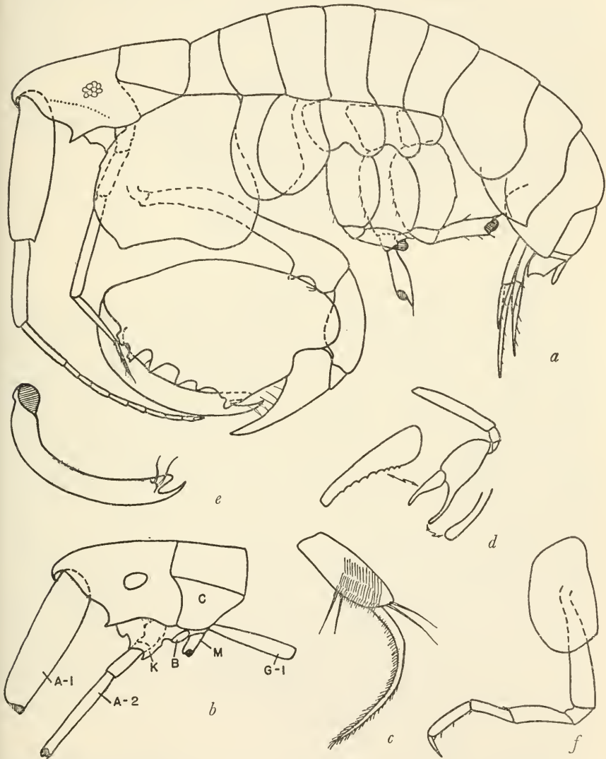
FIGURE 3.— Anamixis falarikia , new species, male, holotype, 2.2 mm., Abbott sta. 145-C-2: a , lateral view; b , view of head (A-1, A-2 = antennae; K = ventral keel; B = bi-lateral bulbs; M = base of maxilliped; C = lateral surface of pereopod segment 1 representing coxa 1; G-1 = base of gnatheopod 1); c , last two articles of maxillipedal palp; d , gnatheopod 1; e , finger of gnatheopod 2; f , pereopod 1.
