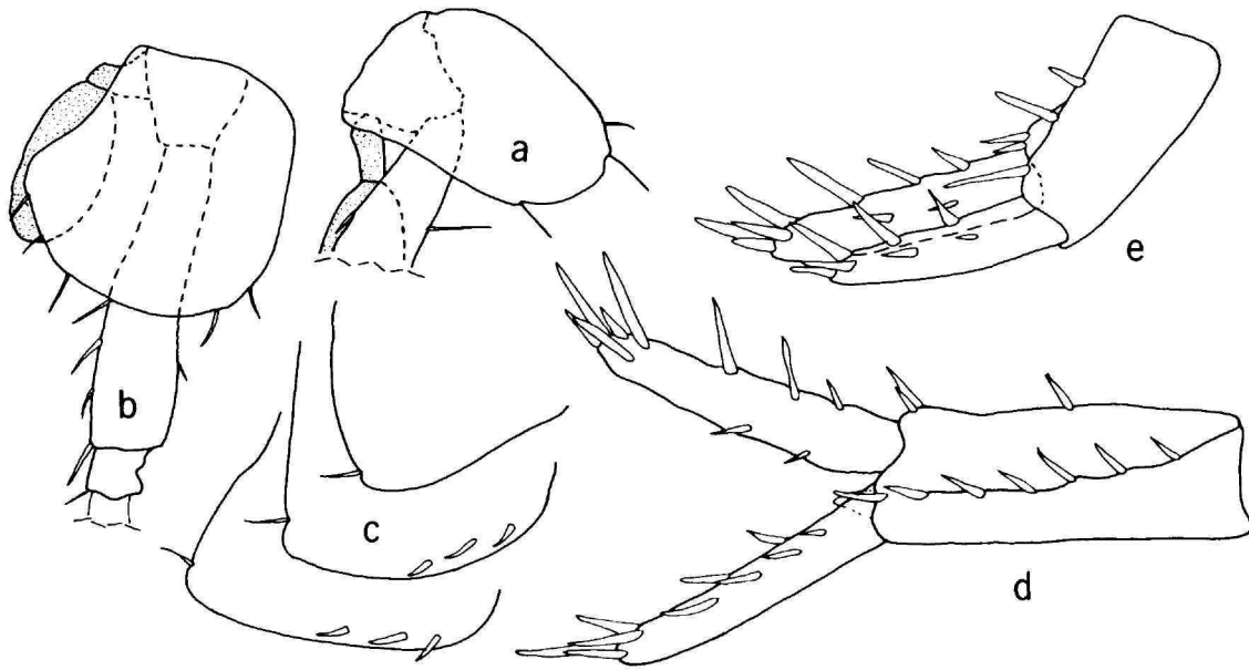
FIGURE 27.— Stygobromus lacicolus , new species, male paratype (5.5 mm): a,b, pereopods 3,4 (in part); c, pleonal plates; d,e, uropods 1,2.
