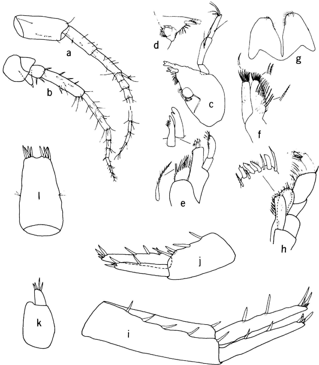
FIGURE 30.— Stygobromus mysticus , new species, female paratype (7.5 mm), Greenview, California: a, b , antennae 1,2; c , right mandible; d , dentate part of left mandible; e, f , maxillae 1,2; g , lower lip; h , maxilliped; i, j, k , uropods 1,2,3; l , telson.
