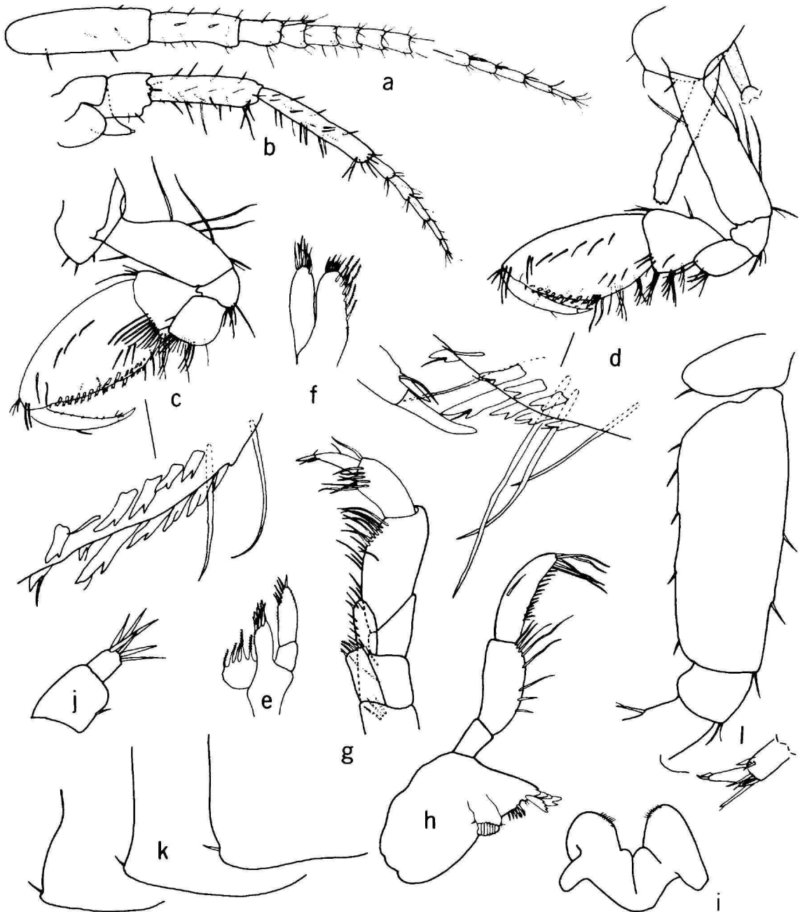
FIGURE 34.— Stygobromus obscurus , new species, female paratype (7.0 mm), well at Victor Crossing, Montana: a,b , antennae 1,2; c,d , gnathopods 1,2; e,f , maxillae 1,2; g , maxilliped; h , left mandible; i , lower lip; j , uropod 3; k , pleonal plates; l , pereopod 7 (in part).
