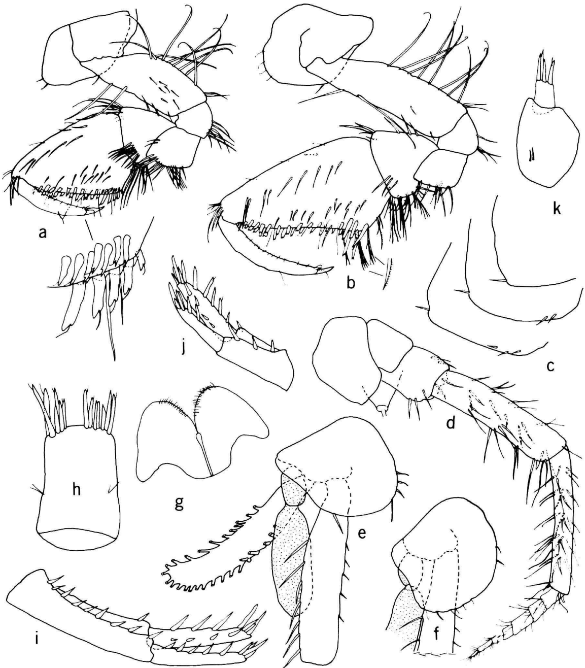
FIGURE 8.— Stygobromus elliotti , new species, female paratype (9.0 mm), Deadhorse Cave, Washington: a, b , gnathopods 1,2; c , pleonal plates; d , antenna 2; e, f , pereopods 3,4 (in part); g , lower lip; h , telson; i, j, k , uropods 1,2,3.
