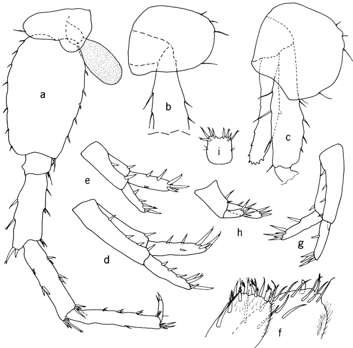
FIGURE 19.— Stygobromus mackenziei , new species. Female paratype (4.7 mm): a, pereopod 6; b,c, pereopods 3,4 (in part); d,e, uropods 1,2; f, apices of inner and outer plates of maxilliped (greatly enlarged). Male paratype (4.0 mm), Empire Cave: g,h, uropods 1,2; i, telson.
