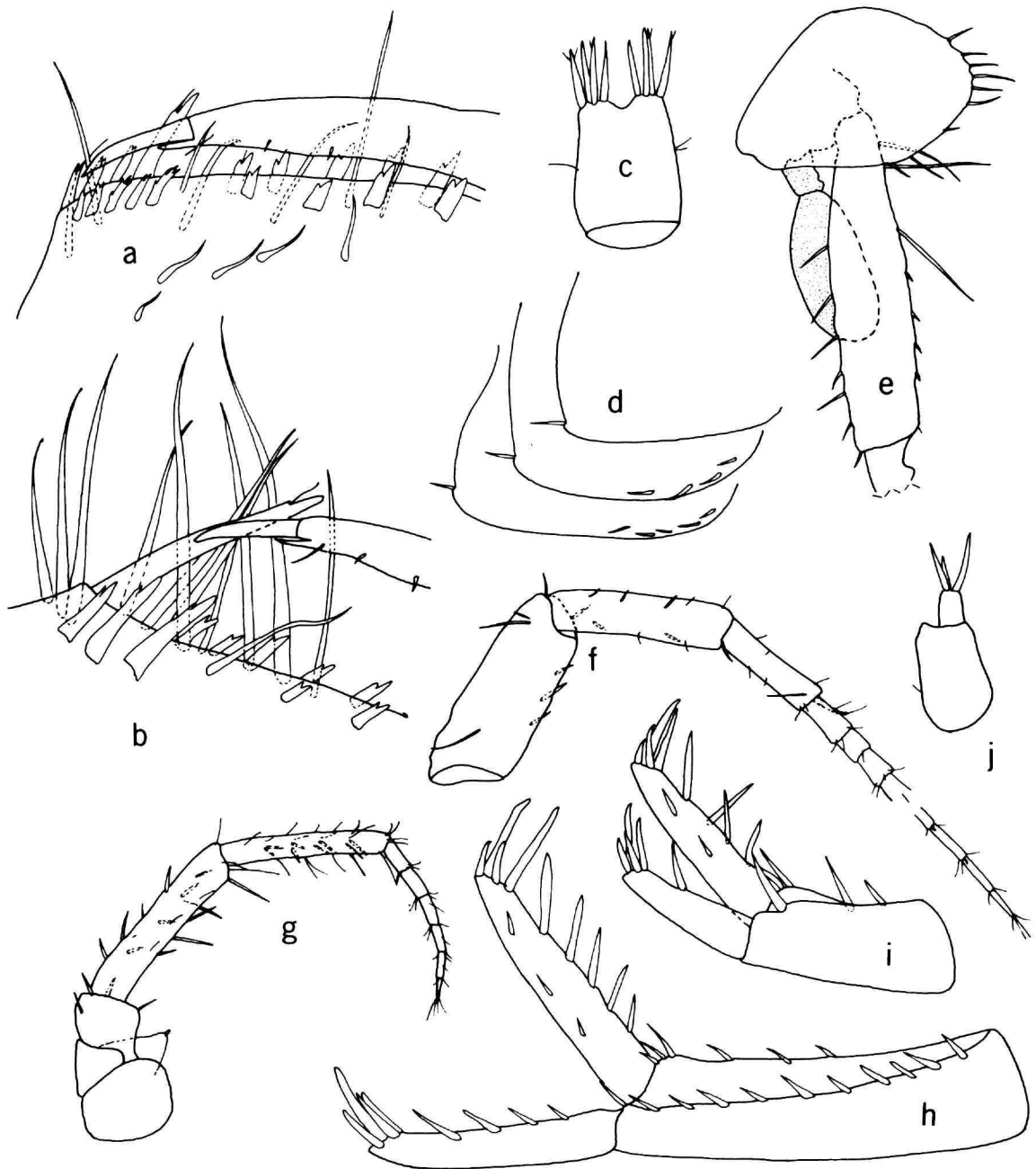
FIGURE 1.— Stygobromus hubbsi Shoemaker, female paratype (6.0 mm), Malheur Cave Oregon: a , b , palms of gnathopodal propods 1,2; c , telson; d , pleconal plates; e , pereopod 3 (in part); f , g , antennae 1,2; h , i , j , uropods 1,2,3.
