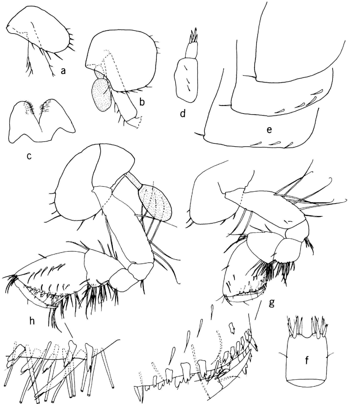
FIGURE 12.— Stygobromus gradyi , new species, female paratype (7.0 mm), Crystal Palace Cave, California: a,b , pereopods 3,4 (in part); c , lower lip; d , uropod 3; e , pleonal plates; f , telson; g,h , gnathopods 1,2.
