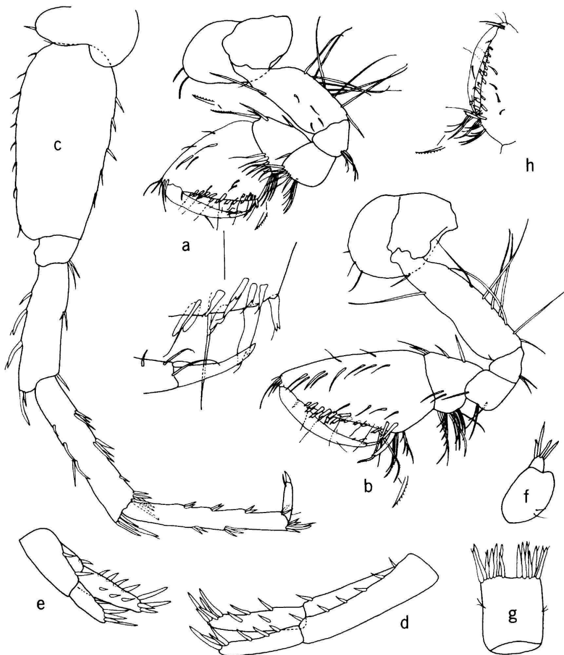
FIGURE 20.— Stygobromus sierrensis , new species. Female paratype (7.0 mm), spring in Trosi Canyon, California: a, b , gnathopods 1, 2; c , pereopod 6; d, e, f , uropods 1, 2, 3; g , telson. Male paratype (5.0 mm), same locality: h , palm of gnathopodal propod 2.
