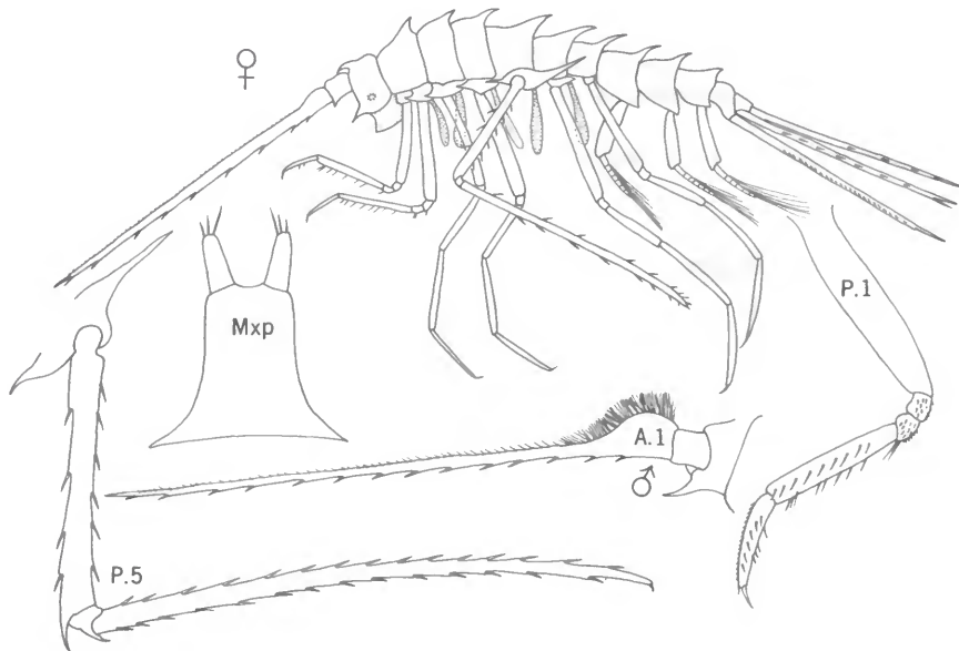
FIGURE 16.— Acanthoscina .
