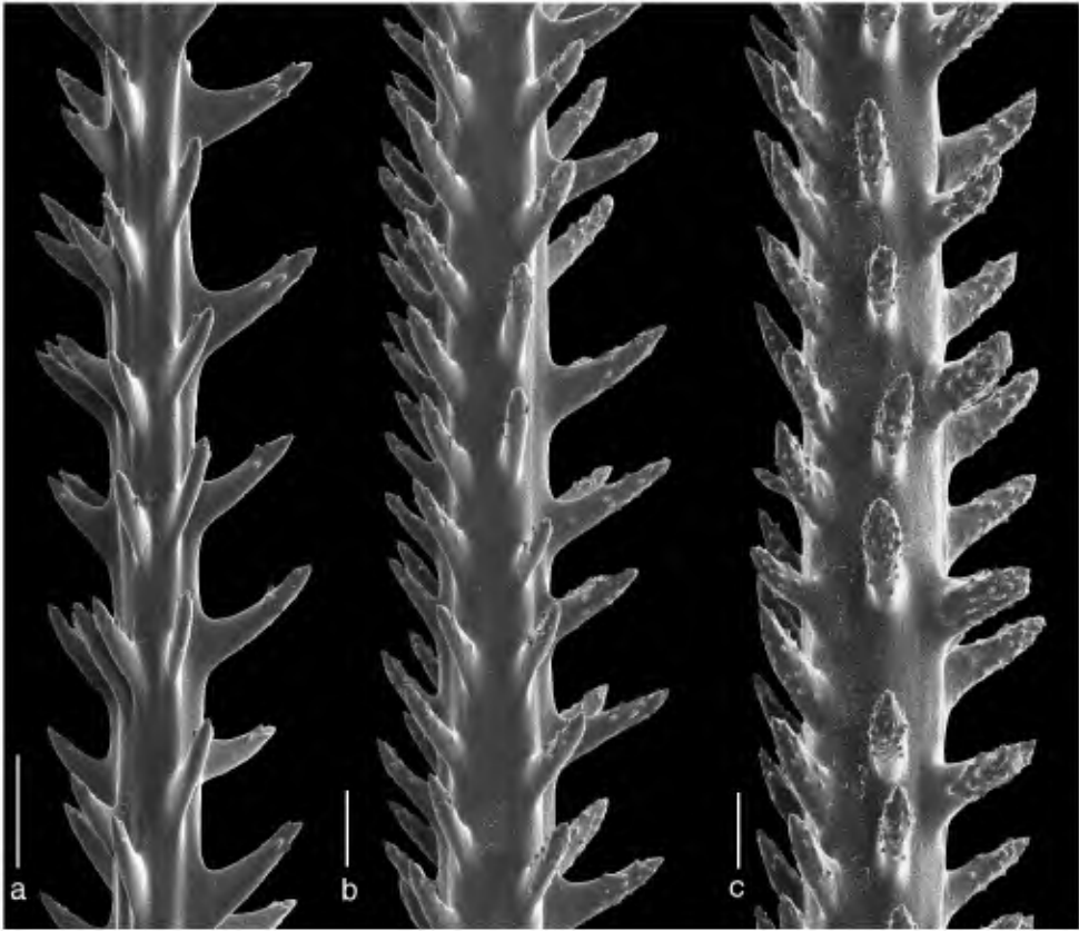
Fig. 4. Pteridopathes pinnata spec. nov., holotype (USNM 1007089); a-c, spines on pinnules, scale 0.1 mm.
