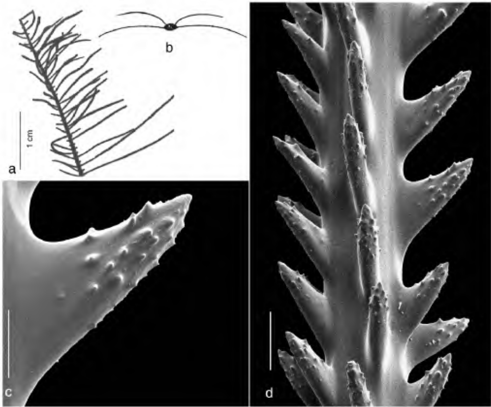
Fig. 6. Tetrathates alata (Brook), holotype (BMNH 1886.2.8.1): a, fragment of the corallum; b, cross-sectional view of branchlet and pinnules, from Brook, 1889, text fig. 19; c, single pinnular spine, scale 0.05 mm; d, spines on pinnule, scale 0.1 mm.
