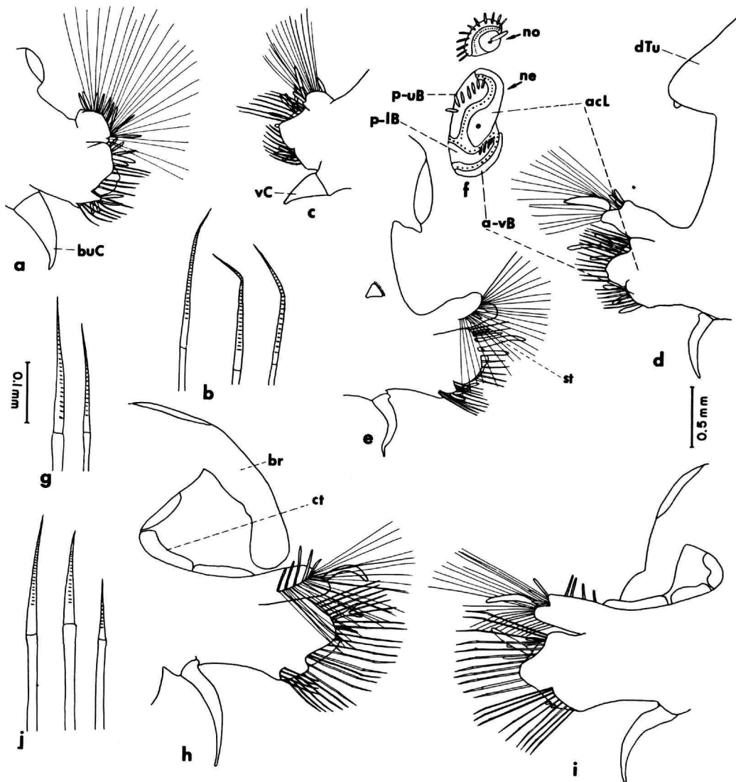
FIGURE 3.— Leanira quatrefagesi (paratype of Leanithalenessa antennata , USNM 40996): a , Parapodium from segment 2, posterior view; b , upper, middle, and lower neurosetae from same; c , parapodium from segment 3, anterior view; d , parapodium from anterior region, anterior view; e , same, posterior view; f , diagrammatic end-view of same, showing position of bracts and setae; g , middle and lower neurosetae from same; h , parapodium from middle region, posterior view; i , same, anterior view; j , upper, middle, and lower neurosetae from same.
