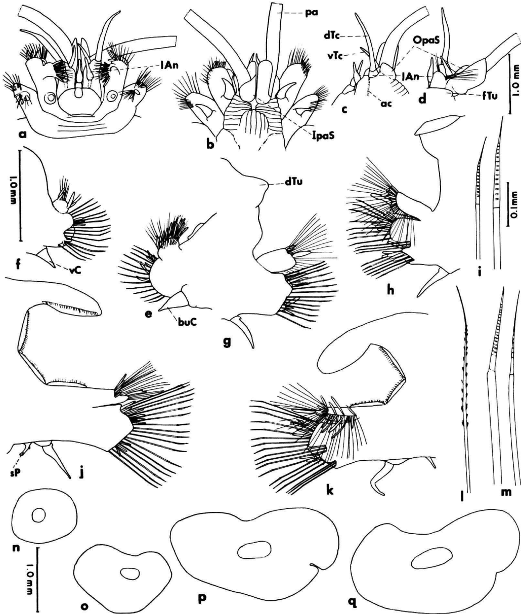
FIGURE 6.— Leanira alba (USNM 41001): a, Anterior end, dorsal view; b, anterior end, ventral view; c, tip of prostomium and right tentacular parapodium, outer or lateral view; d, left tentacular parapodium, inner or medial view; e, parapodium from segment 2, anterior view; f, parapodium from segment 3, posterior view; g, parapodium from anterior region, anterior view; h, same, posterior view; i, middle and lower neurosetae from same; j, parapodium from middle region, anterior view; k, same, posterior view; l, upper simple neuroseta from same; m, middle and lower neurosetae from same; n, right second elytron; o, right third elytron; p, right elytron from anterior region; q, right elytron from middle region.
