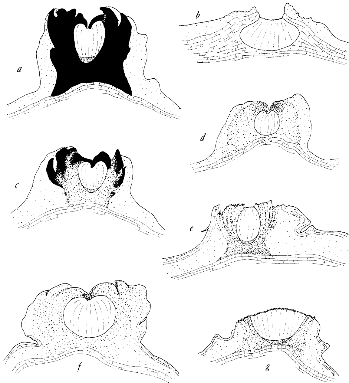
FIGURE 8.—Cross sections of apothecia of Graphina : a, G. acharii (lectotype in G); b, G. cf. adscribens (Wirth 519); c, G. antillarum (Duss s.n.); d, G. carneoviridis (Hale 37642); e, G. chlorocarpa (lectotype in G); f, G. colliculosa (lectotype of G. eugeniae , Merrill 3471); g, G. colliculosa (lectotype in PC).
