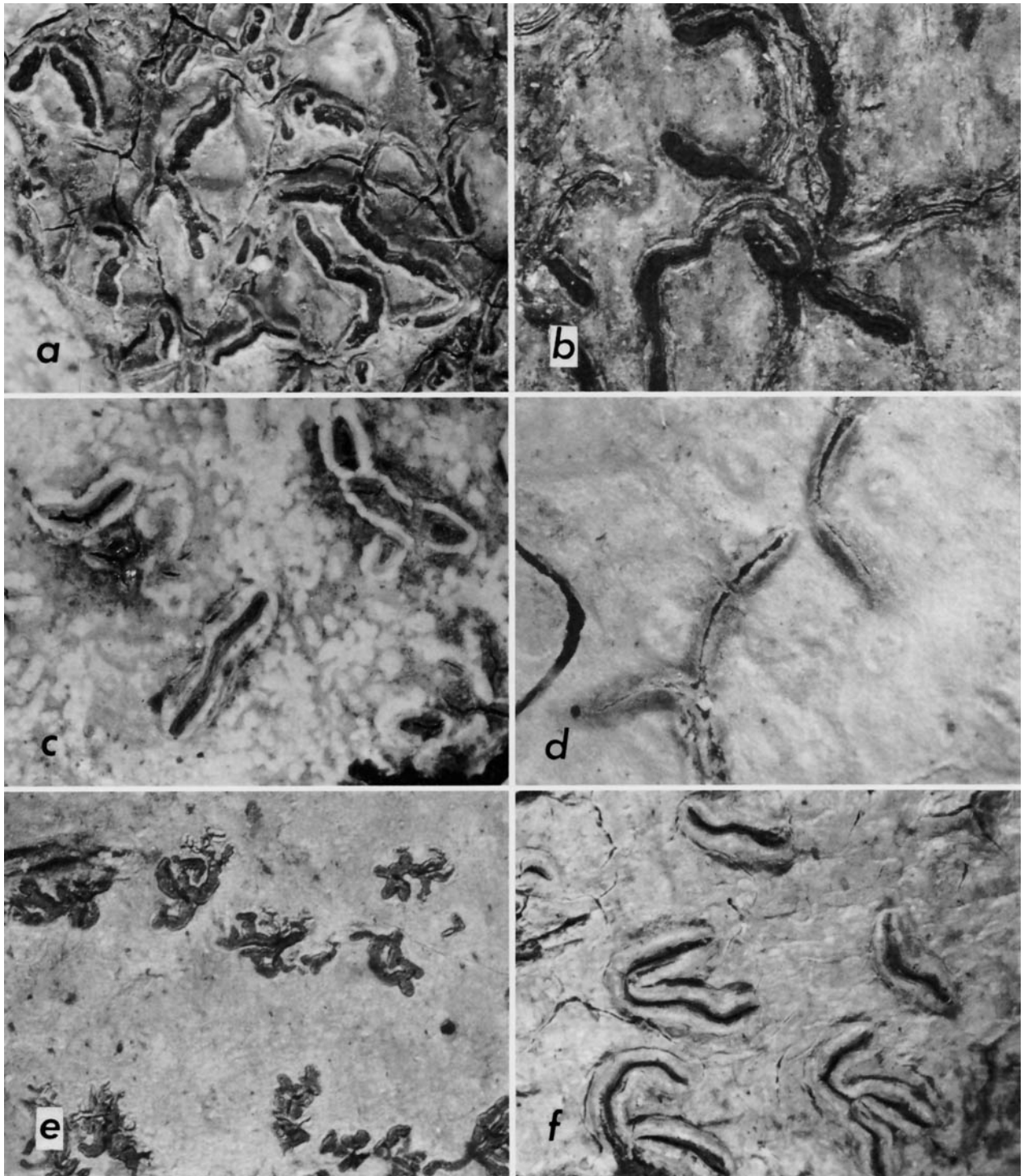
PLATE 6.—Species of Phaeographis and Graphina : a, P. exaltata (Hale 35321); b, P. haematites (Hale 38013); c, P. mordenii (Hale 35071); d, P. rosea (Elliott in BM); e, P. subtigrina (Wirth 444); f, G. acharii (Hale 35555).
