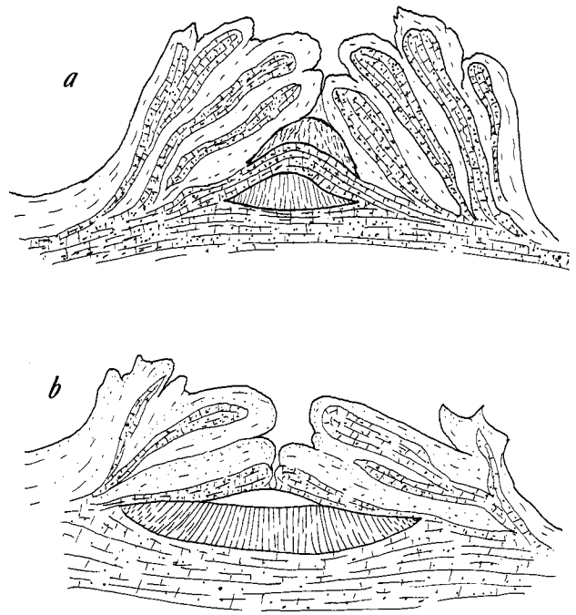
FIGURE 1.—Cross sections of Graphina peplophora from Mexico: a, Wirth 150; b, Wirth 361.
