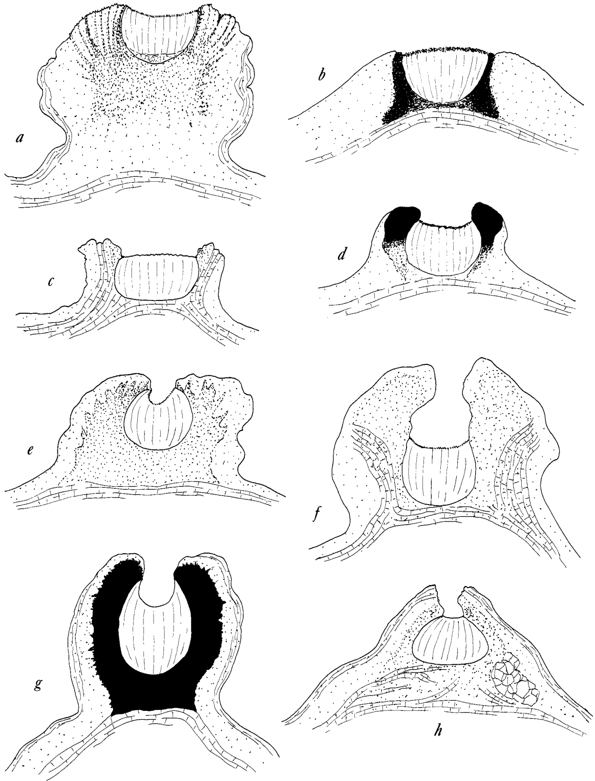
FIGURE 9.—Cross sections of apothecia of Graphina : a, G. colliculosa (lectotype of G. aibonitensis Fink); b, G. collospora (Boergesen s.n.); c, G. columbina (Beaumont s.n.); d, G. dimidiata (Vainio 332); e, G. dispersa (Malme 2038B); f, G. frumentaria (lectotype in G); g, G. illinata (lectotype in M); h, G. incrustans (lectotype in G).
