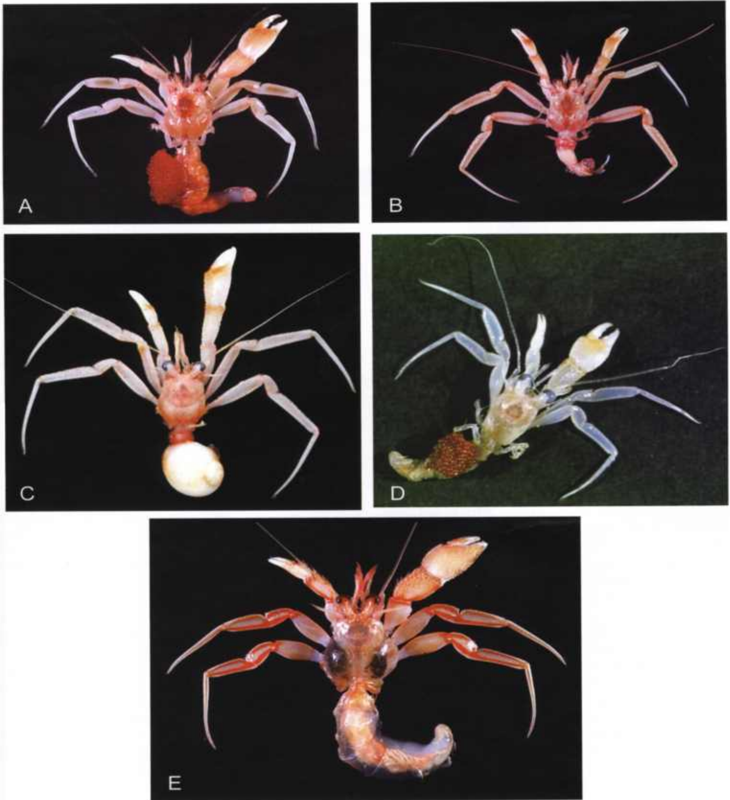
Fig. 8.— Live coloration. A-D, Strobopagurus gracilipes (A. Milne-Edwards, 1891): A, ov F 5.1 mm, TAIWAN 2003, stn CP 214 (NTOU A00001); B, M 6.0 mm (with abnormal right cheliped), same station (NTOU A00001); C, M 6.1 mm, French Polynesia, BENTHAUS, stn CP 1965 (MNHN Pg 6594); D, ov F 3.8 mm, French Polynesia, BENTHAUS, stn DW 1863 (MNHN Pg 7003). E, Strobopagurus sibogae (de Saint Laurent, 1972): F 6.2 mm, TAIWAN 2003, stn CP 216 (NTOU A00007). Photographs by T.-Y. Chan (A, B, E), and J. Poupin (C, D).
