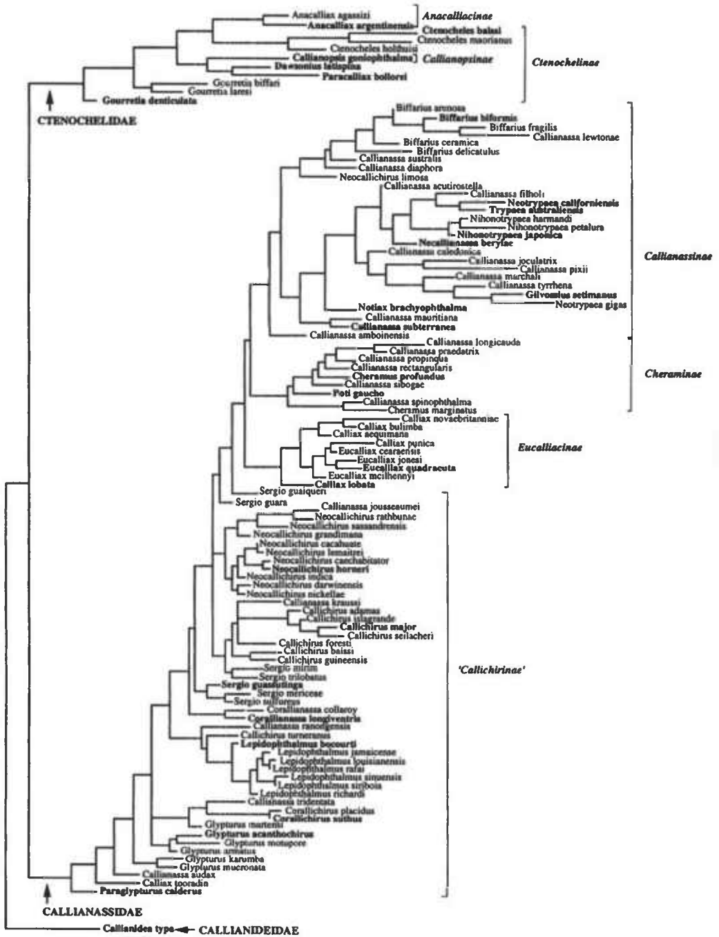
Fig. 3. Phylogram of 50% majority rule consensus tree of 1,700 equally parsimonious trees obtained from an heuristic analysis of 107 thalassinidean taxa using 93 morphological characters and using the out-group method. Tree length = 838 steps; consistency index (CI) = 0.905. Some higher taxonomic categories are indicated (arrows and brackets), as are type species (boldface).
