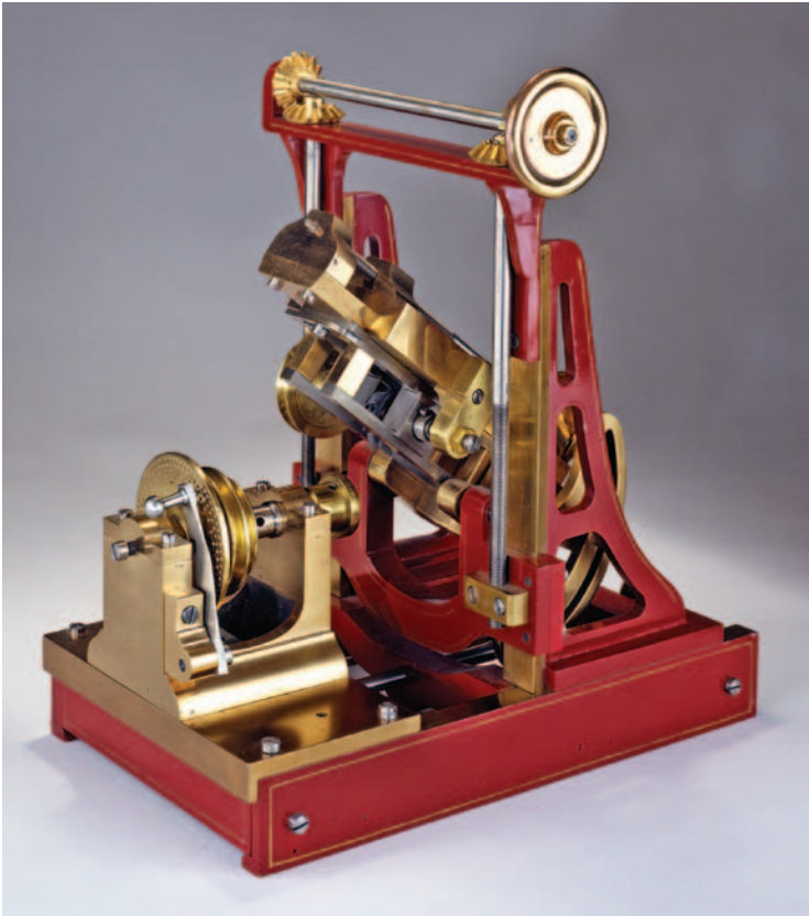
Patent No. 153,370. John A. Peer. Gear Cutting Machine. July 21, 1874. (SI neg. 86-6311)
