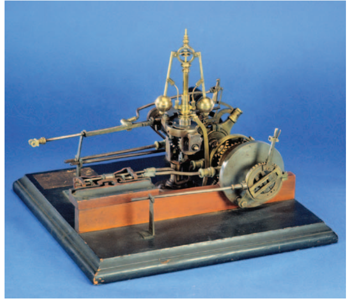
Patent No. 220,151. Mathias L. Jacquemin. Valve Regulating Mechanism. September 30, 1879. (SI neg. 89-6764)
