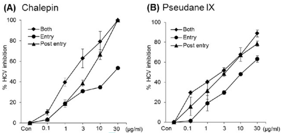
4 Fig. 3. Mode-of-action analysis of chalepin and pseudane IX. Huh7.5 cells infected with HCV were treated with various concentrations of chalepin (A) and pseudane IX (B) at different timings; (i) only during virus inoculation (entry), (ii) only after virus inoculation (post entry) and (iii) both during and after virus inoculation (both), with a total incubation time of 48 h. Con, control. Percent inhibitions at each concentration and IC 50 values are shown. The data represent mean ± SEM of data from two independent experiments.
