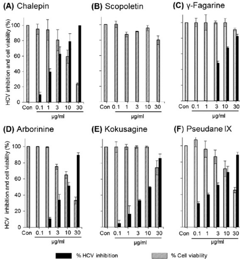
71 Fig. 2. Dose-dependent inhibition of HCV infection by isolated compounds and their cytotoxicity. Various concentrations of isolated compounds, chalepin (A), scopoletin (B), γ-fagarine (C), arborinine (D), kokusagine (E) and pseudane IX (F), were mixed with an equal amount of HCV to obtain a final concentration of 30 to 0.1 µg/ml and inoculated to Huh 7.5 cells (MOI = 0.5). After virus adsorption, the cells were cultured with the same concentrations of compounds for 46 h. The culture supernatants were harvested and titrated for virus infectivity. Percent inhibitions of HCV infectivity by each compound are shown. In parallel, cytotoxicity of the compounds was measured by WST-1 assay. Con, control. The data represent means ± SEM of data from two independent experiments.
