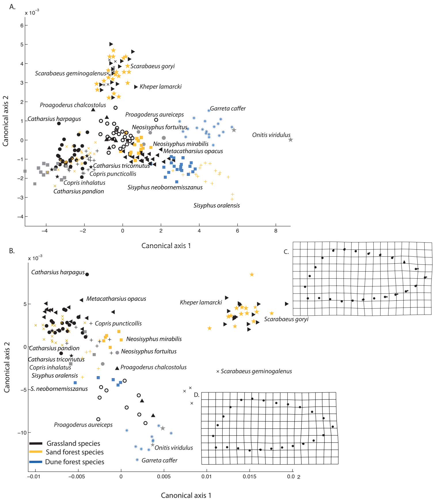
Fig S1. Ordination plot for canonical axes 1 and 2 representing differences in morphology between the RA4 and CuJ vein regions in 17 Scarabaeinae species. A. RA4 vein region. B. CuJ vein region (veins CuA plus J). C and D. Deformation grids for variation on CVA 1 with respect to the consensus shape for (C) RA4 and (D) CuJ.
