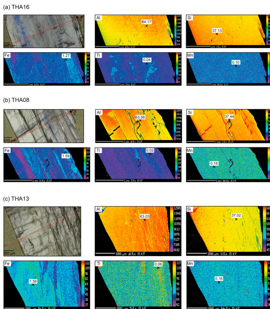
Figure 12. Electron probe microanalyses (EPMA) semi-quantitative X-ray maps of Al, Si, Fe, Ti and Mn on the \langle 100 \rangle faces of blue-green THA16 (a), yellow THA08 (b) and orange THA13 (c) kyanite samples, with color scales expressed in counts, not calculated to concentration. The red line corresponds to the EPMA quantitative profile analyses (Table S12d–f). The maximum values (in oxide wt. %) measured along the profile for a given element is reported on each map.
