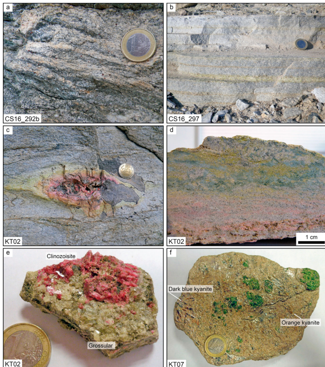
Figure 3. (a) Main garnet–kyanite–biotite–hematite–plagioclase \pm staurolite \pm sillimanite bearing gneiss of the Trikorfo area (sample CS16_292b, N290/65N). (b) Green epidote-rich horizon parallel to the main gneiss foliation (sample CS16_297, N270/11N). (c) Lense slightly oblique to the subhorizontal gneiss foliation showing a zonation of green epidote and pink clinozoisite together with grossular in a geode (sample KT02). (d) Mineralogical zonation with diopside, hornblende, epidote (green), grossular and clinozoisite (pink-red), sample KT02 equivalent to Th04. (e) Close up to the core of the geode to near gem-quality pink clinozoisite (clinothulite) and grossular association within locality sample KT02. (f) Deep green Mn-rich andalusite (viridine) and kyanite (deep blue and orange) association in sample KT07.
