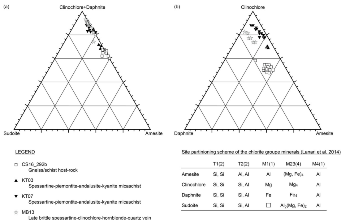
Figure A1. Composition of chlorite-group minerals analyzed by EPMA in (a) Clinochlore + Daphnrite–Sudoite–Amesite and (b) Clinochlore–Daphnrite–Amesite ternary plots. The mineral names are according to the site partitioning scheme used in Lanari et al. [97].
