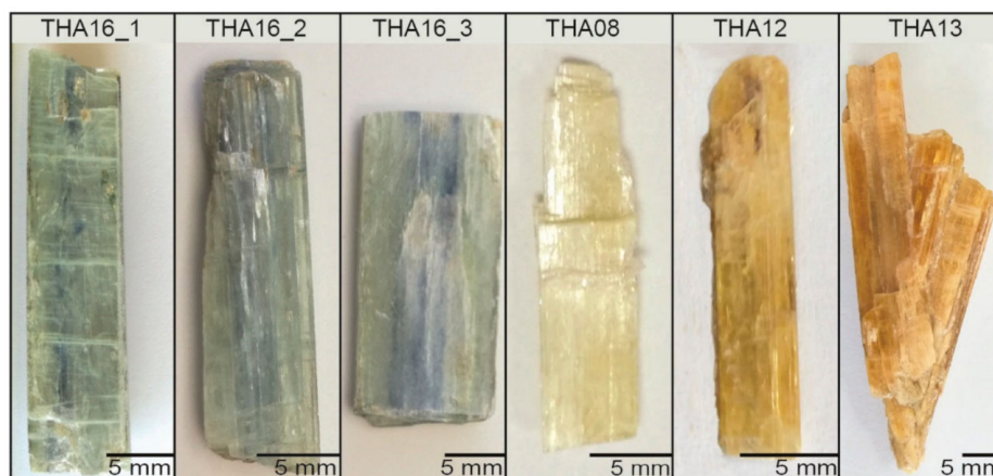
Figure 8. Photographs of individual kyanite crystals prior to bulk rock analyses.
