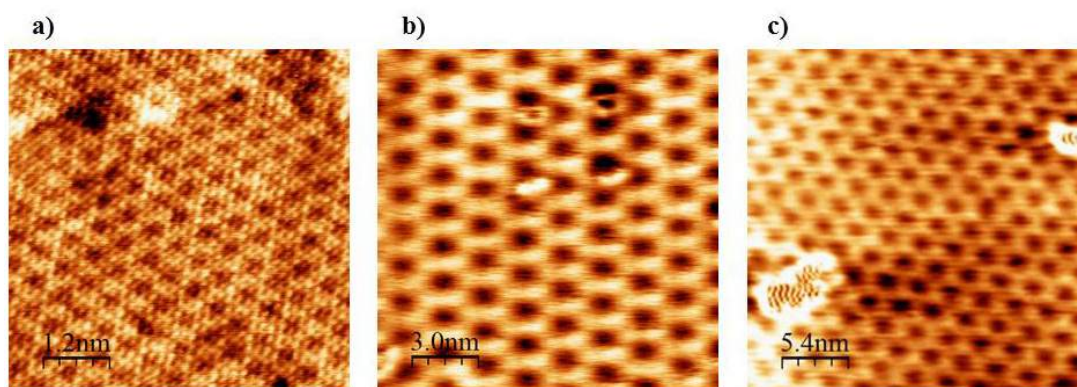
Figure V.28. STM images of SLG grown from C_{60} on: (a) Pt(111), ( 6 \times 6 ) nm, 0.11 V, 2.3 nA. (b) Ir(111), ( 15 \times 15 ) nm, 1.2 V, 2.6 pA and (c) Cu(111), ( 27 \times 27 ) nm, -0.4 V, 2.7 pA. In every image different moiré superstructures are shown.
