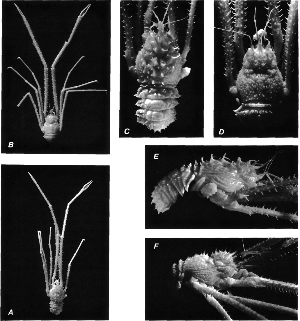
Fig. 2. Comparison of a specimen of Gastroptychus formosus (Filhol, 1885) (A, C, E) with the holotype of G. salvadori new species (B, D, F). A, B dorsal view; C, D dorsal view; E, F lateral view. A, C, E: female (carapace length including rostrum, 20 mm) collected off north-west Spain, 42°15'N, 11°22'W, Discovery Stn. 9042, 1541–1662 m, Discovery Collections, Institute of Oceanographic Sciences Deacon Laboratory, Wormley, U.K.
