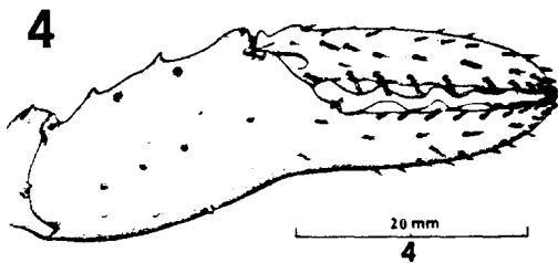
FIGURE 4. Lithodes nintokuae Sakai, off Oahu, Hawaii. Male CL 59 mm. Hand of right cheliped, outer surface.
