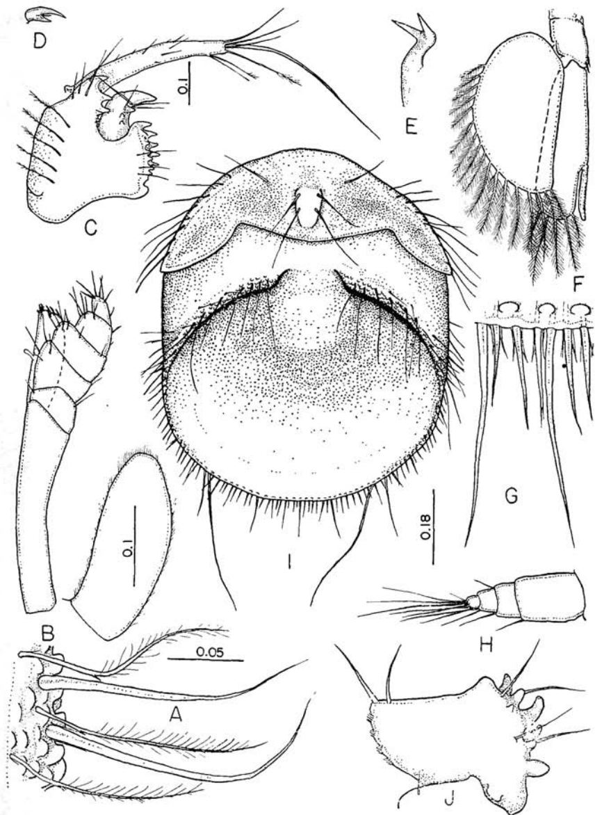
FIGURE 35. Limnoria (L.) insulae , new species, male. A, lateral crest of pleotelson. B, maxilliped. C, uropod. D, accessory claw of first pereopod. E, laciniod seta of right mandible. F, second pleopod. G, posterior edge of pleotelson. H, flagellum of second antenna. I, pleotelson. J, merus of first pereopod. Figures with similar magnification, A, D, G, H, J; B; C, F, I; E.
