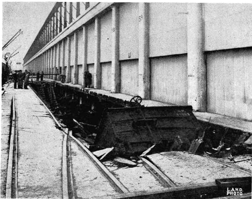
FIGURE 1. Collapse of creosoted wooden piles due to attack by Limnoria tripunctata at Berth 59, Los Angeles Harbor. Piles had been in service only 12-13 years. Photo courtesy of Los Angeles Harbor Department, via Mr. Carrol M. Wakeman, Testing Engineer.
