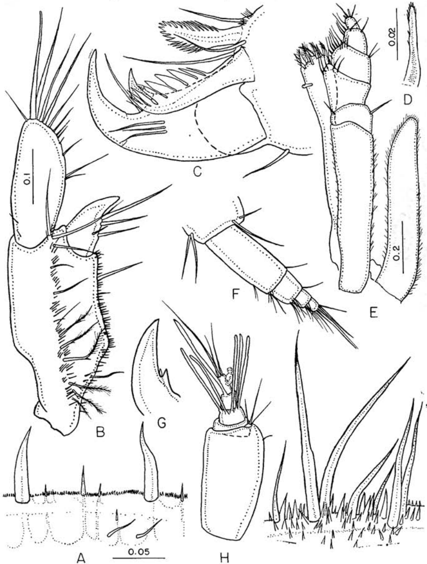
FIGURE 41. Linnoria (P.) stephensi , new species, female. A, distal margin of pleotelson. B, uropod. C, distal parts of first pereopod. D, lacinoid seta of right mandible. E, maxilliped. F, flagellum of second antenna. G, accessory claw, first pereopod. H, distal articles of first antenna, note epizootic protozoan. I, lateral crest of pleotelson. Figures with similar magnification, A, C, H; B, F, G; D; E.
