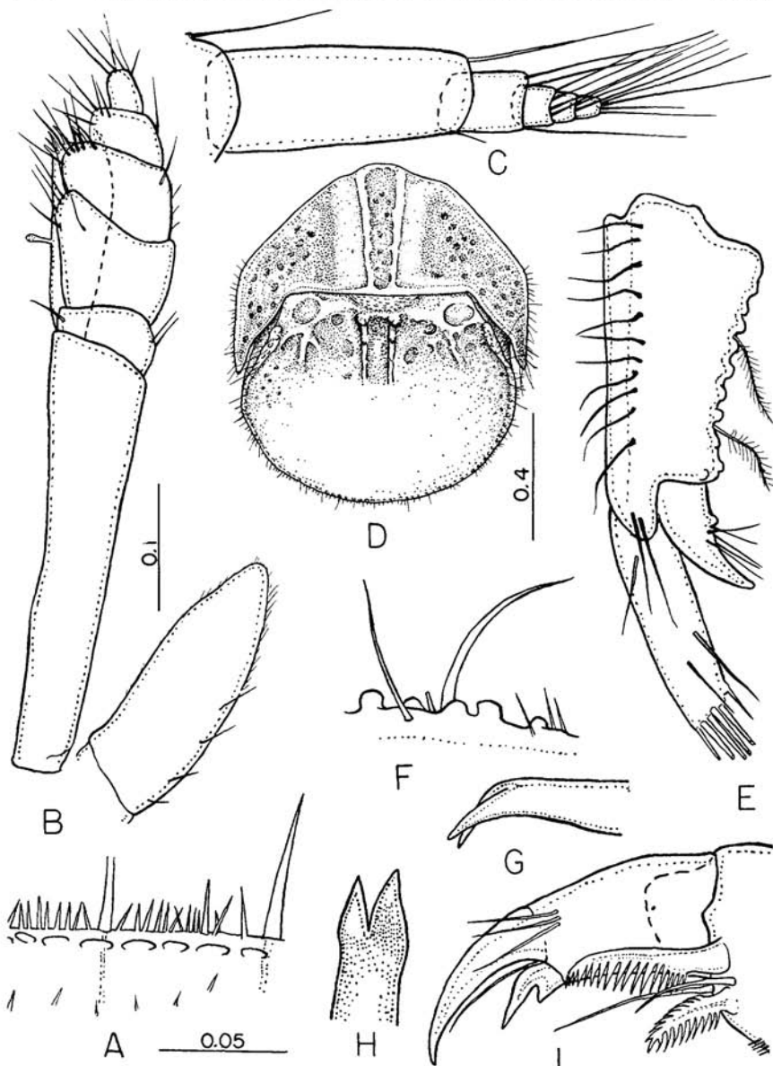
FIGURE 18. Limnoria ( L. ) saseboensis , new species, paratype. A, posterior margin of pleotelson. B, maxilliped. C, flagellum of second antenna. D, pleotelson. E, uropod. F, lateral crest of pleotelson. G, lacinioid seta of right mandible, lateral view. H, lacinioid seta of right mandible, medial view. I, distal articles of first pereopod. Figures with similar magnification, A, F, I; B, C, E; D-, H, G (magnification not known).
