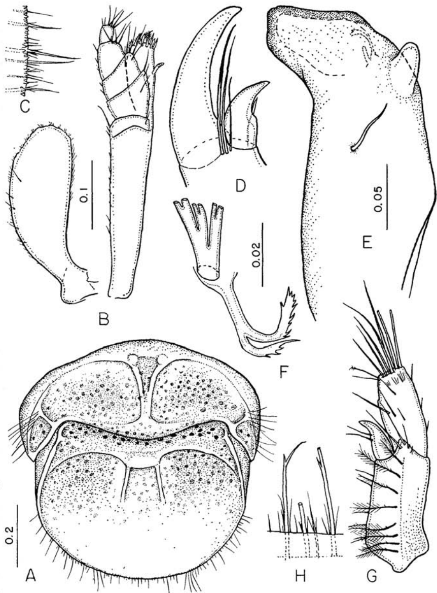
FIGURE 38. Limnoria (P.) segnoides , new species. A, pleotelson. B, maxilliped. C, posterior margin of pleotelson. D, distal parts of first pereopod. E, outer surface of left mandible. F, lacinioid seta and setal row of right mandible. G, uropod. H, lateral crest of pleotelson. Figures with similar magnification, A; B, G; C, E, H; D, F.
