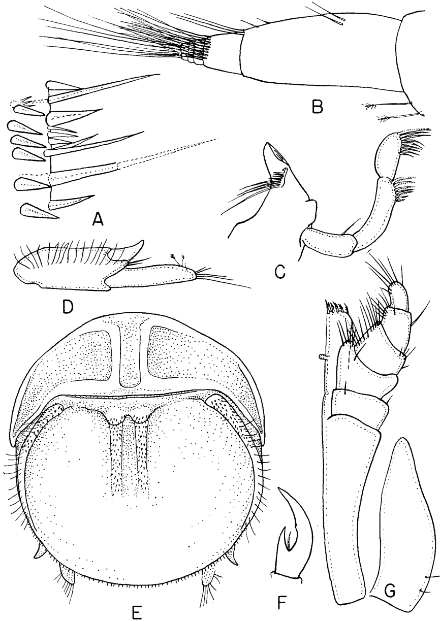
FIGURE 34. Limnoria (L.) sublittorale , new species, male paratype. A, posterior border of pleotelson. B, flagellum of second antenna. C, right mandible. D, uropod. E, pleotelson. F, accessory claw of dactyl of first pereopod. Magnification, scales various, all taken from paratype 4 mm in length and 1.2 mm in width of pleotelson.
