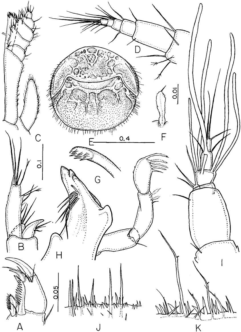
FIGURE 40. Limnoria (P.) rugosissima , new species, male paratype. A, distal article of first pereopod. B, uropod. C, maxilliped. D, flagellum of second antenna. E, pleotelson. F, seta of penultimate article of mandibular palp. G, laciniod seta of right mandible. H, right mandible inner surface. I, distal articles of first antenna. J, distal margin of pleotelson. K, lateral crest of pleotelson. Figures with similar magnification, A, D, H, I, J, K; B, C; E, F, G.
