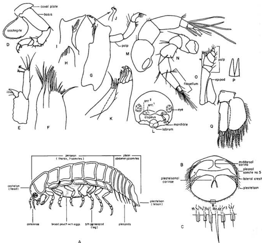
FIGURE 6. The external morphology of Limnoria . A, lateral view of gravid female (after G. O. Sars, 1897, and Menzies, 1954). B, Fifth pleonal somite and pleotelson. C, posterior border of pleotelson highly magnified. D, Leg of gravid female with attached oostegite. E, Uropod. F, First maxilla. G, right mandible of wood-borer. H, incisive part of right mandible of wood-borer, showing "file." I, Left mandible of wood-borer showing "rasp." J, Lacinioid seta of right mandible. K, Second maxilla. L, Frontal view of head. M, First antenna. N, Second antenna. O, Maxilliped. P, Penes (genital appophyses). Q, Second pleopod of male.
