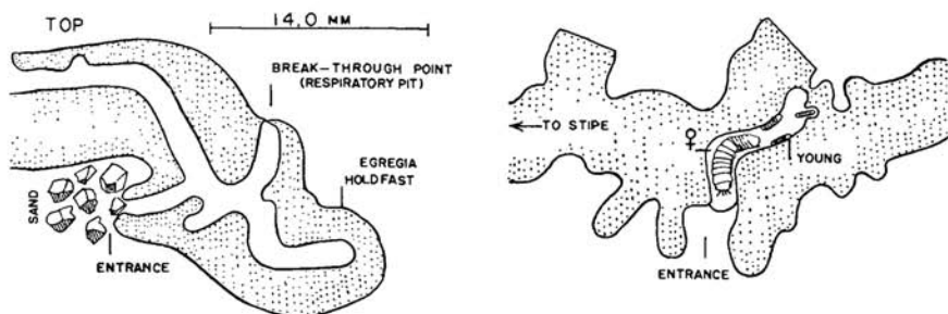
FIGURE 4. A sketch of the attack by Limnoria on the hold-fast of the seaweed Egregia .
