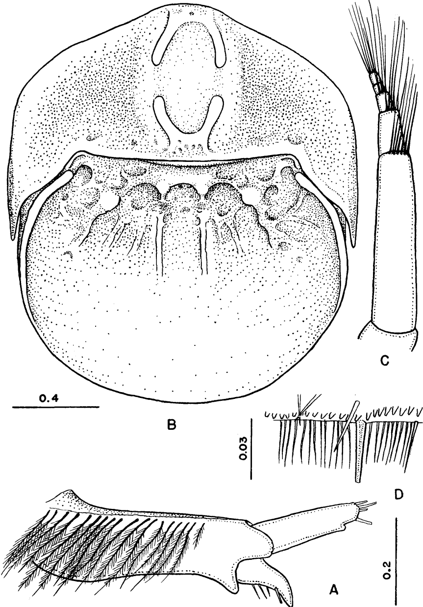
FIGURE 29. Limnoria (? L. ) septima Barnard, female cotype. A, uropod. B, pleotelson. C, flagellum of second antenna. D, posterior edge of pleotelson. Figures with similar magnification, A, C; B; D.
