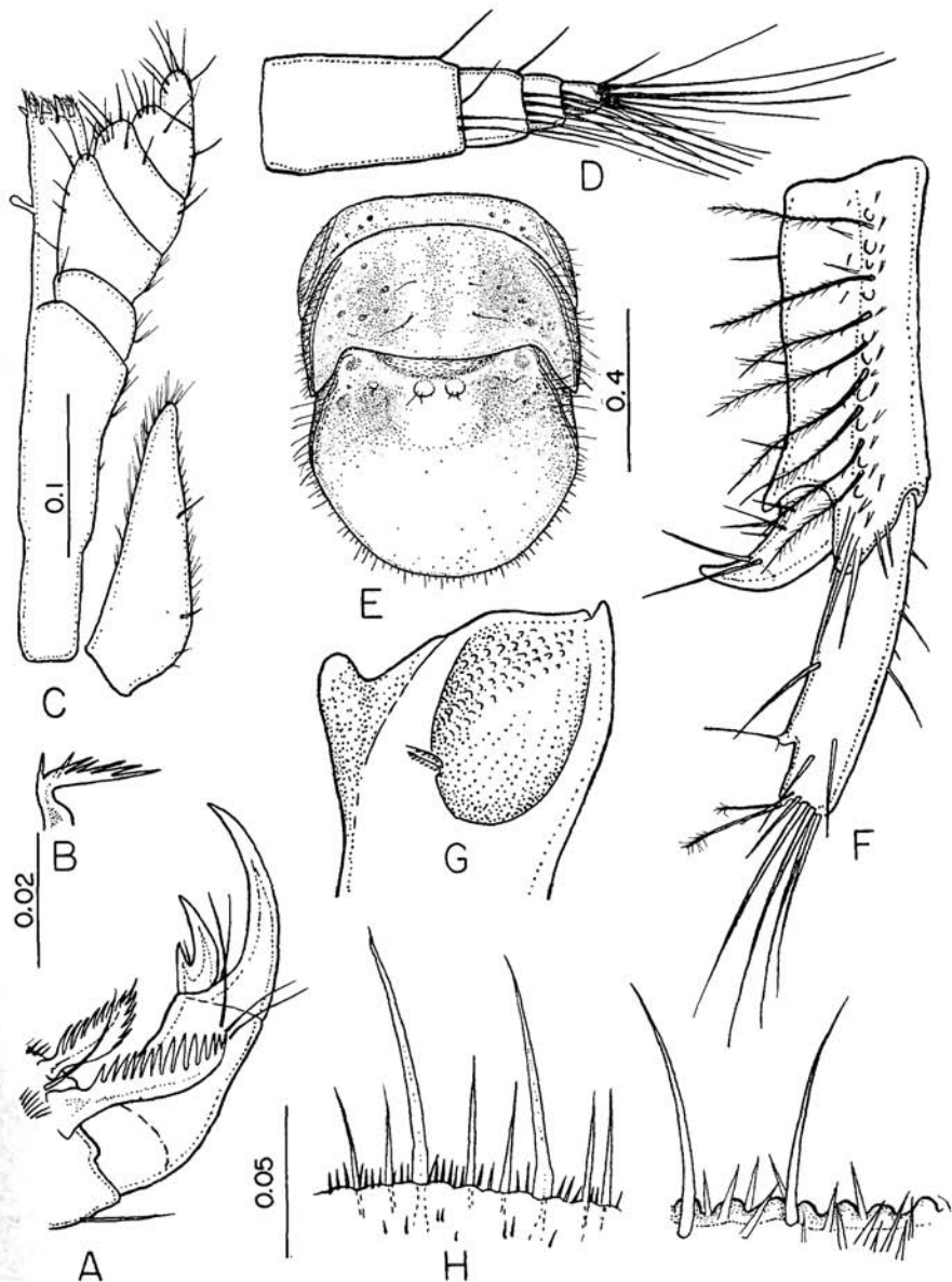
FIGURE 19. Limnoria (L.) simulata , new species, male paratype. A, distal articles of first peraeopod. B, laciniod seta of right mandible. C, maxilliped. D, flagellum of second antenna. E, pleotelson. F, uropod. G, inner surface of left mandible, palp not shown. H, posterior margin of pleotelson. I, lateral crest of pleotelson. Figures with similar magnification, A, D, G, H, I; B; C-, E.
