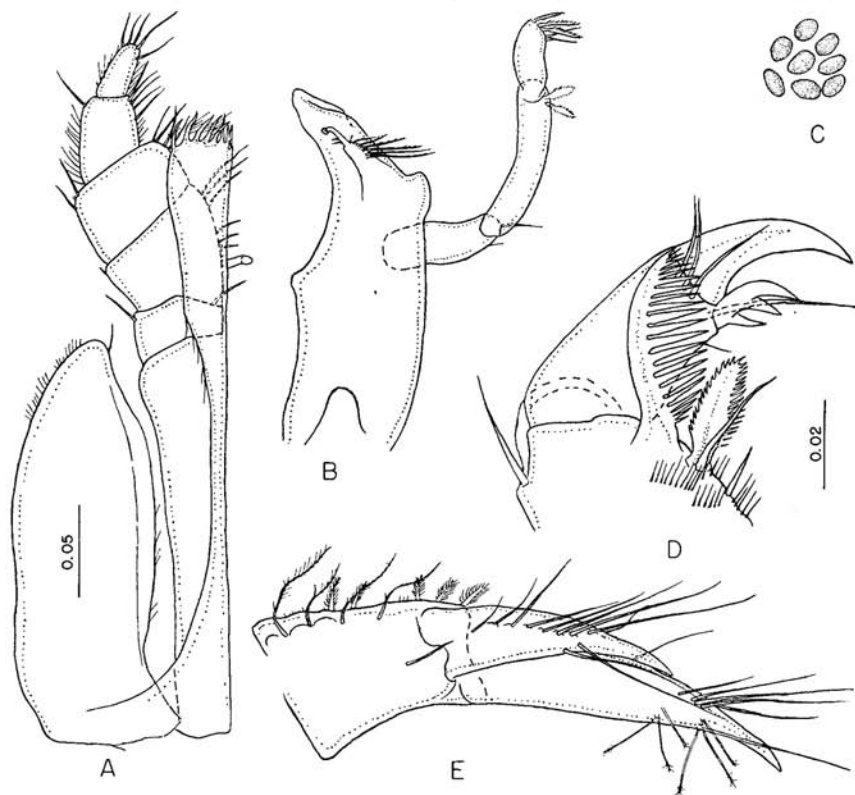
FIGURE 23. Paralimnoria andrewsi (Calman). A, maxilliped. B, right mandible. C, eye, lateral view. D, distal articles of first pereopod. E, uropod. Figures with similar magnification, A, B, C, E; D.
