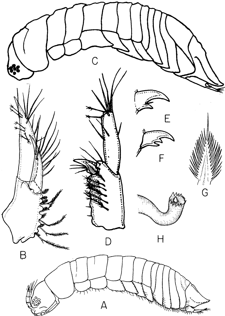
FIGURE 7. The distinguishing features of the genera of the Limnoriidae. A, Paralimnoria , lateral view. B, Uropod of Paralimnoria . C, Limnoria , lateral view. D, Uropod of Limnoria . E, Dactyl of first pereiopod of Limnoria . F, Dactyl of first pereiopod of Paralimnoria . G, Peculiar setae of peduncle of uropod of Paralimnoria . H, Lacinioide seta of mandible of Paralimnoria .
