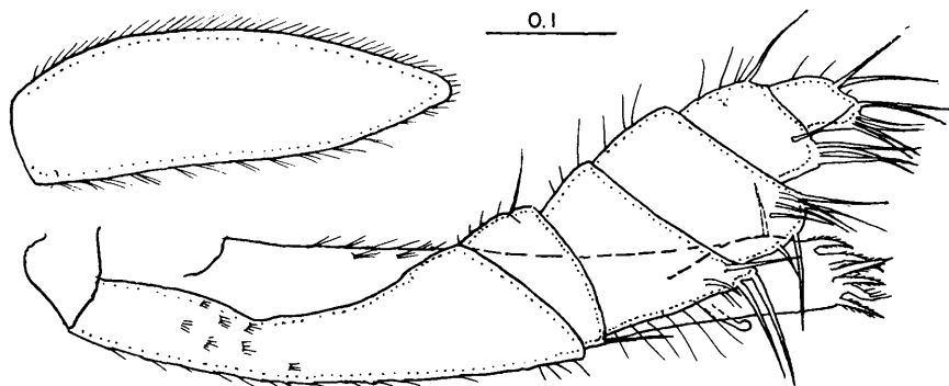
FIGURE 21. Limnoria (P.) algarum , new species, paratype, maxilliped.
