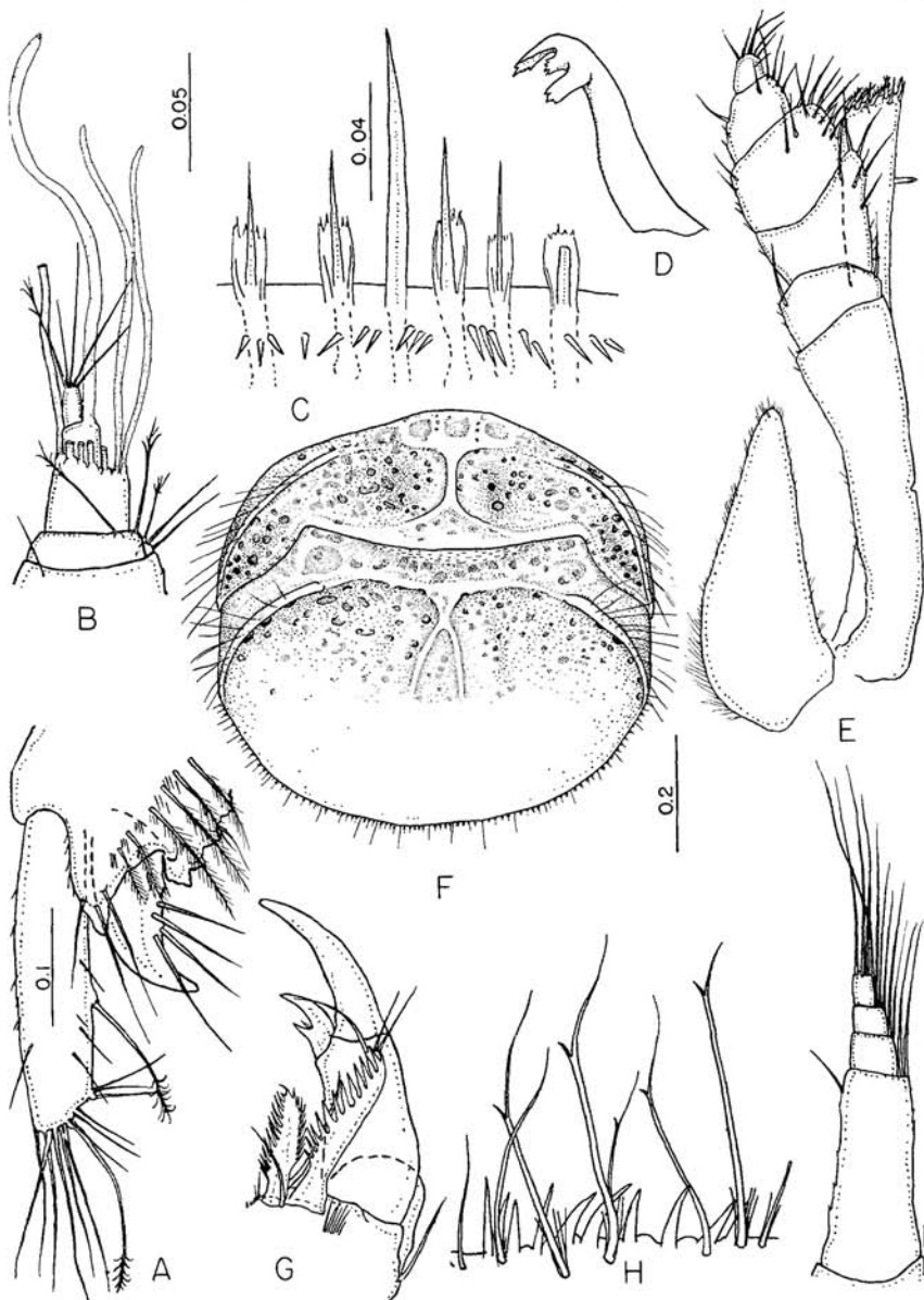
FIGURE 9. Limnoria (L.) lignorum (Rathke), topotypic male. A, distal parts of uropods. B, distal article of first antenna. C, apex of pleotelson. D, lacinioid seta of right mandible. E, maxilliped. F, pleotelson. G, distal parts of first pereopod. H, lateral crest of pleotelson. I, flagellum of second antenna. Figures with similar magnification, A, E; B, G, H, I; C-, D-, F.
