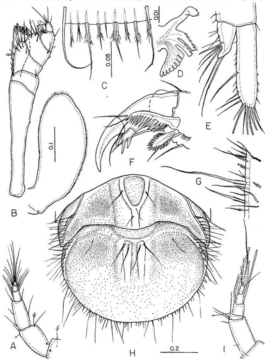
FIGURE 15. Limnoria (L.) pfefferi Stebbing, female cotyope. A, second antenna. B, maxilliped. C, posterior edge of pleotelson. D, setal row and lacinoid seta of right mandible. E, uropod, distal parts. F, first peraeopod, distal parts. G, lateral crest of pleotelson. H, pleotelson, dorsal view. I, first antenna. Figures with similar magnification, A, B, E, F, I; C, G; H; D.
