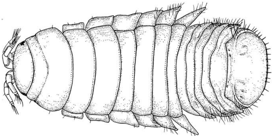
FIGURE 42. Limnoria (P.) stephenseni , new species, female slightly compressed, pleotelson foreshortened slightly, length of female 7.5 mm.
