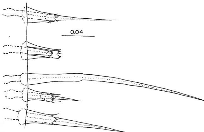
FIGURE 28. Pleotelsonic border of L. (L.) japonica Richardson.
