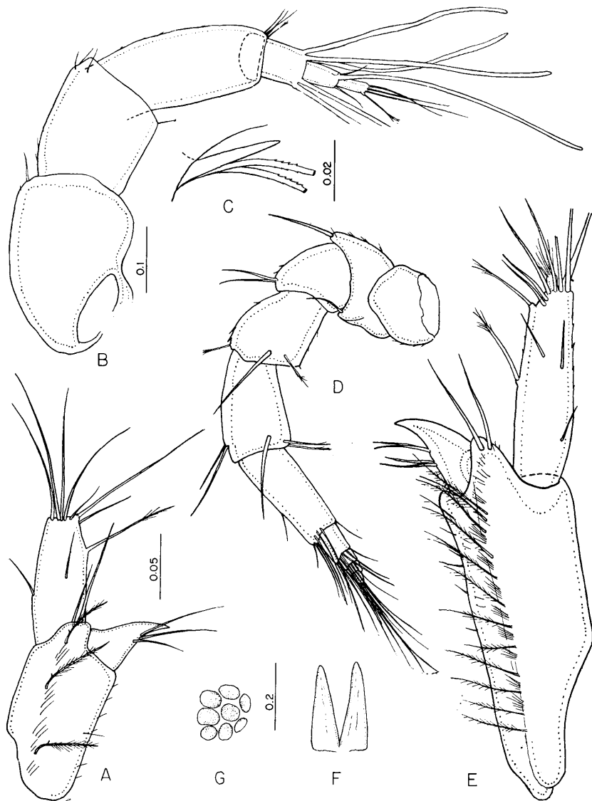
FIGURE 12. Limnoria (L.) quadripunctata Holthuis. A, uropod, juvenile, 1.0 mm length. B, first antenna. C, setal row of left mandible. D, second antenna. E, uropod. F, genital apophyses. G, eye, lateral view. Figures with similar magnification, A; B, D, E, F; C; G.
