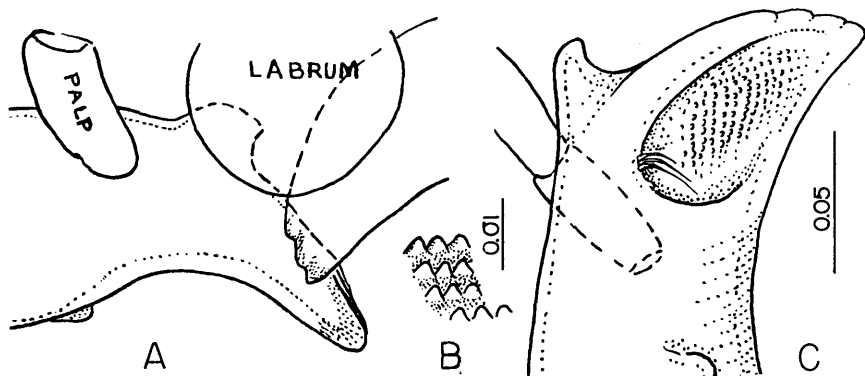
FIGURE 8. Mandibles of Paralimnoria . A, frontal view. B, "rasp" on inner surface of left mandible. C, inner surface of left mandible.
