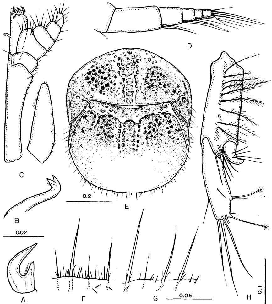
FIGURE 33. Limnoria (L.) foveolata , new species, holotype. A, accessory claw of first pereopod. B, lacinioid seta of right mandible. C, maxilliped. D, flagellum of second antenna. E, pleotelson. F, uropod. G, posterior margin of pleotelson. H, lateral crest of pleotelson. Figures with similar magnification, B; D, H; E; F, G; A and C not known.
