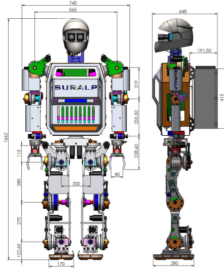
Fig. 9. SURALP, dimensions.
