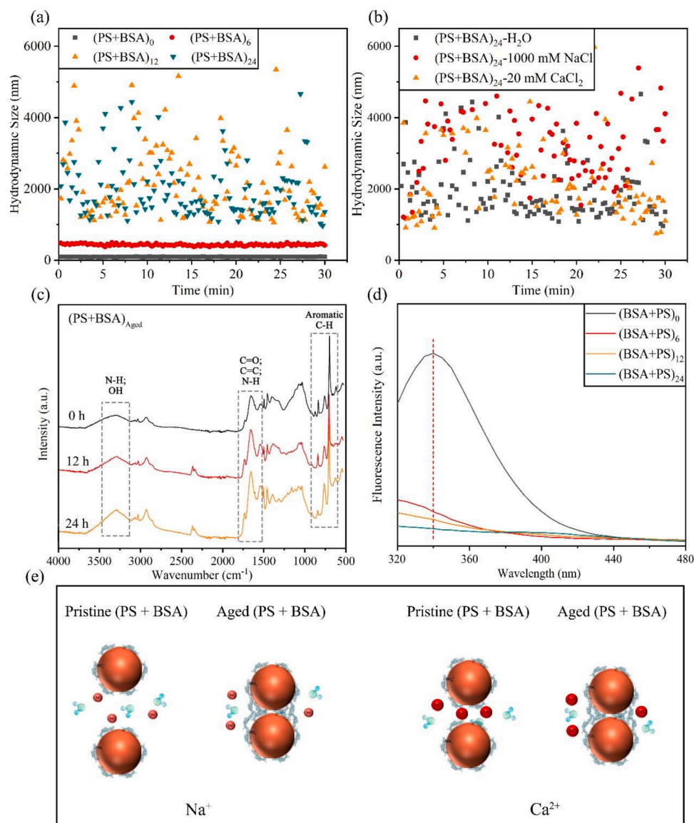
Fig. 5. The effect of photoaging on the aggregation kinetics of PS NPs with BSA in NaCl (a) and \text{CaCl}_2 (b) solutions; The FTIR (c) and fluorescence (d) spectra of PS NPs with BSA; Schematic diagram of the effect of photoaging on the stability of BSA associated PS NPs (e). Subscripts 0, 6, 12 and 24 mean aging times of 0, 6, 12 and 24 h.
