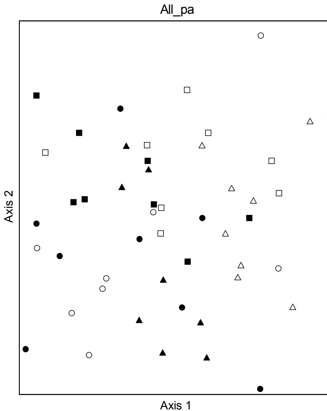
Figure 5.5 Ordination based on the bird species sighted revealed slight clustering at the property level but not between burnt and unburnt sites. Circles = Roxmere, Squares = Bushy Park, Triangles = Carlton Hills, Black = burnt sites and white = unburnt sites.
