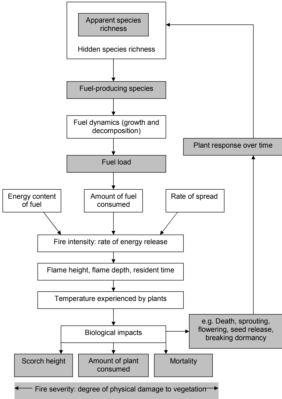
Figure 3.2 A generalised diagram showing the relationship between fire and vegetation.
