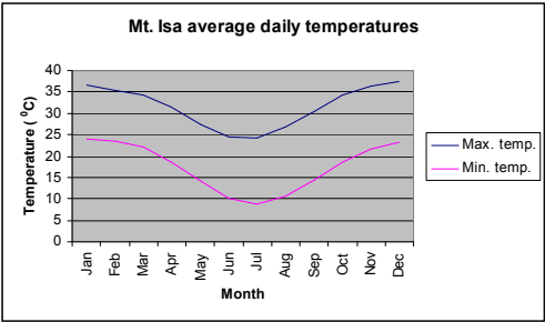
Figure 2.3 Annual temperature range (difference between the summer maximum and winter minimum) and the average annual temperatures in the Mount Isa Inlier. Map based on Bioclim data (EPA 2003); line graphs based on Clewett et al. (2003).
