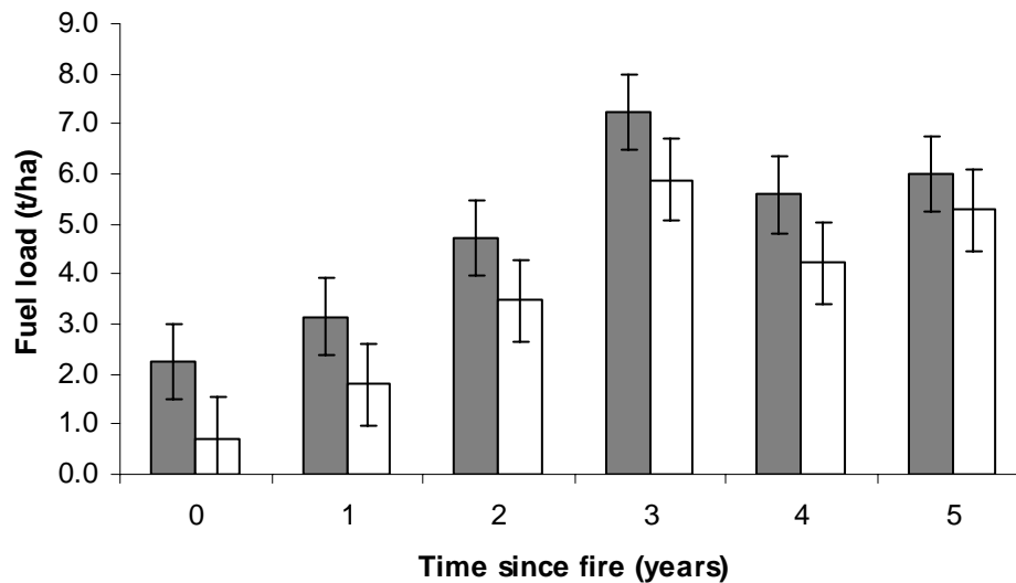
Figure 4.19 On average, the regression model over-predicted fuel load by 0.7 to 1.5 t/ha across all fire ages. (Grey bars = predicted average, white bars = actual average, error bars = standard error).
