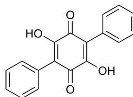
Fig. 33 Classes of lichen substances which are derived by shikimate pathway
