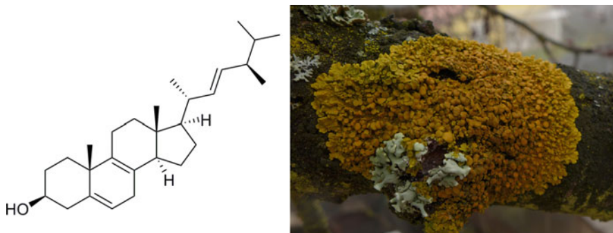
Fig. 29 Lichesterol structure ( Xanthoria parietina )
