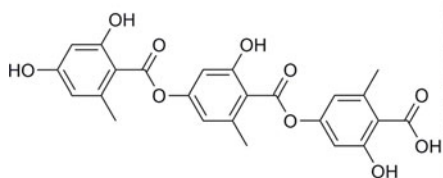
Fig. 8 Gyrophoric acid structure ( Lasallia pustulata )
