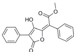
Fig. 36 Vulpinic acid structure ( Vulpicida pinastri )
