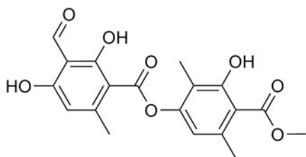
Fig. 9 Atranorin structure ( Hypogymnia tubulosa )
