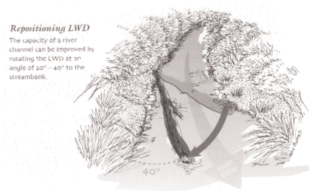
Figure 8: Repositioning large woody debris (Gippel et al, 1998).
