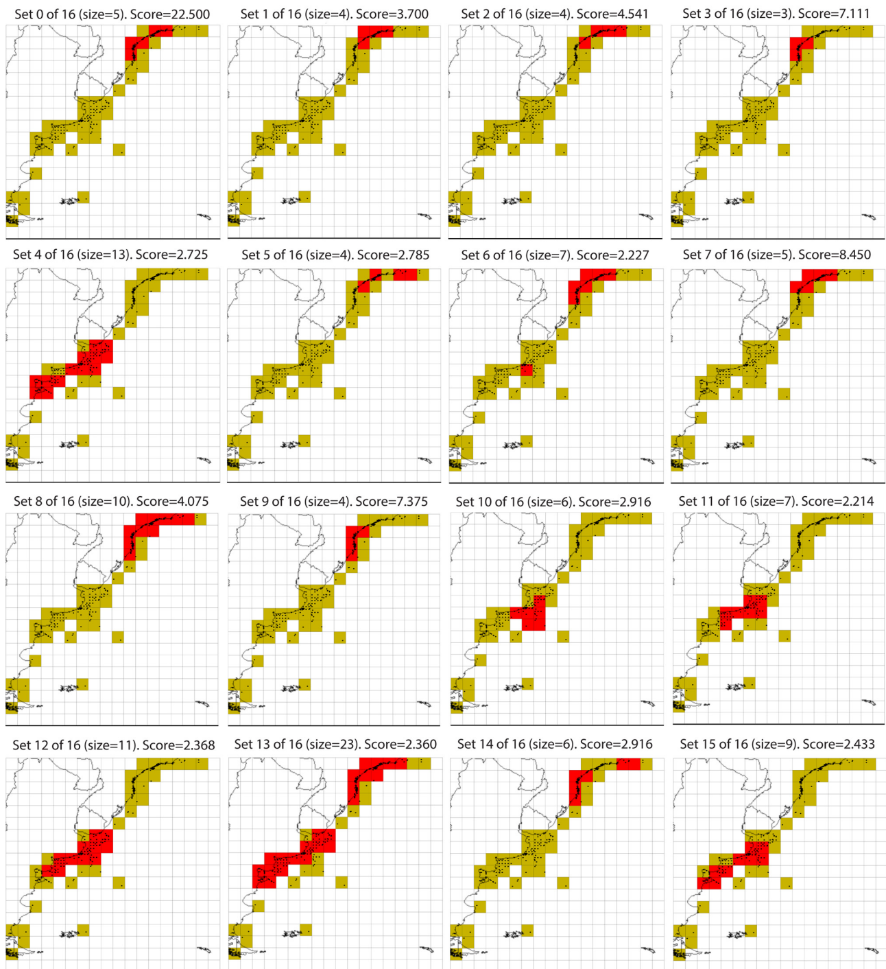
FIGURE 1. Areas of endemism (in red), their number of quadrants (size) and their score, in sets 0 to 15 resulting from the EA with NDM VNDM for quadrants 2^{\circ}\times 2^{\circ} and F = 0.5 . In yellow are the quadrants with benthic hydroids occurrences considered by the NDM VNDM for the EA.
