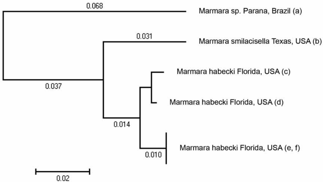
FIG. 111. Sequence distance tree of Marmara derived from 6 samples among 3 species based upon neighbor-joining analysis with Kimura 2-parameter model. The analysis shows significant COI divergences among the North American Marmara smilacisella reared from Smilax (b), the apparently undescribed Marmara reared from Schinus terebinthifolius in Brazil (a), as well as Marmara habecki mostly reared from Schinus in Florida, USA (c–f). Sequence lengths are shown on main branches. Pertinent specimen data including source of tissue samples for each specimen are: (a) Brazil: Parana: 13 km W Curitiba, larva, host: Schinus terebinthifolius ; (b) USA: Texas: Harris Co: Houston, adult legs, host: Smilax sp.; (c) USA: Florida: Pinellas Co: Fort Desoto Park, adult legs, host: Schinus sp.; (d) USA: Florida: Polk Co: entire moth, Lake Alfred, from Marmara gulosa pheromone trap; (e, f) USA: Florida: Broward Co: Fort Lauderdale, larvae, host: Schinus terebinthifolius .
