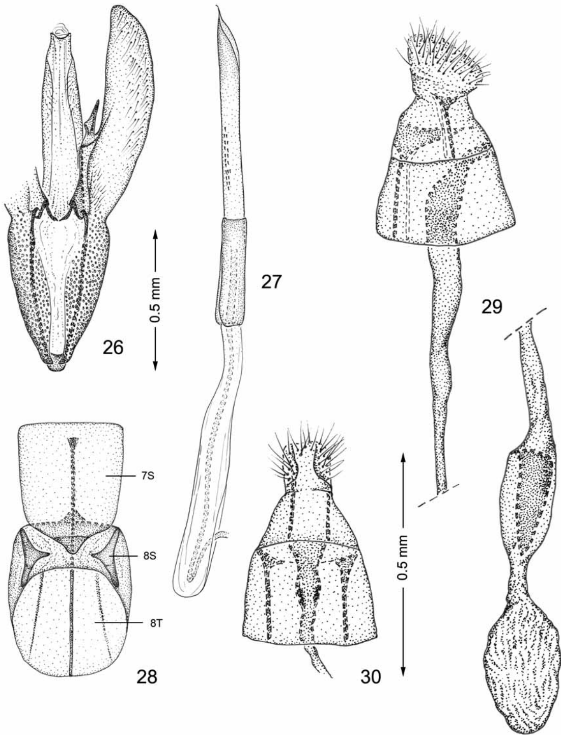
FIGS. 26–30. Eucosmophora schinusivora , genitalia and postabdomen. 26. Male, ventral view. 27. Aedeagus. 28. Male postabdominal segments 7–8, ventral view. 29. Female, lateral view. 30. Female, ventral view. (Scale lengths as indicated).
