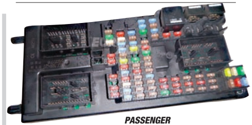
PASSENGER COMPARTMENT FUSE BOX - YQE500420SW
