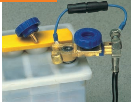
'DIS-CAR-NECT' STARTER IMMOBILISER RX1356 REPLACEMENT SCREW KNOB RX1356K REPLACEMENT FUSE RX1356F
