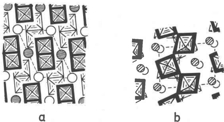
FIG. 7. (a) Idealized octahedral drawing of ThTi_2O_6 projected onto (010). Th atoms are large open circles. (b) Triclinic BiNbO_4 projected onto (010). Bi atoms are large open circles.
