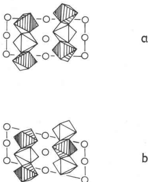
FIG. 6. (a) SbNO_4 ; (b) \beta-Sb_2O_4 . Shown as assemblages of octahedra projected onto (010). Sb atoms not octahedrally coordinated to oxygen atoms are shown as open circles.
