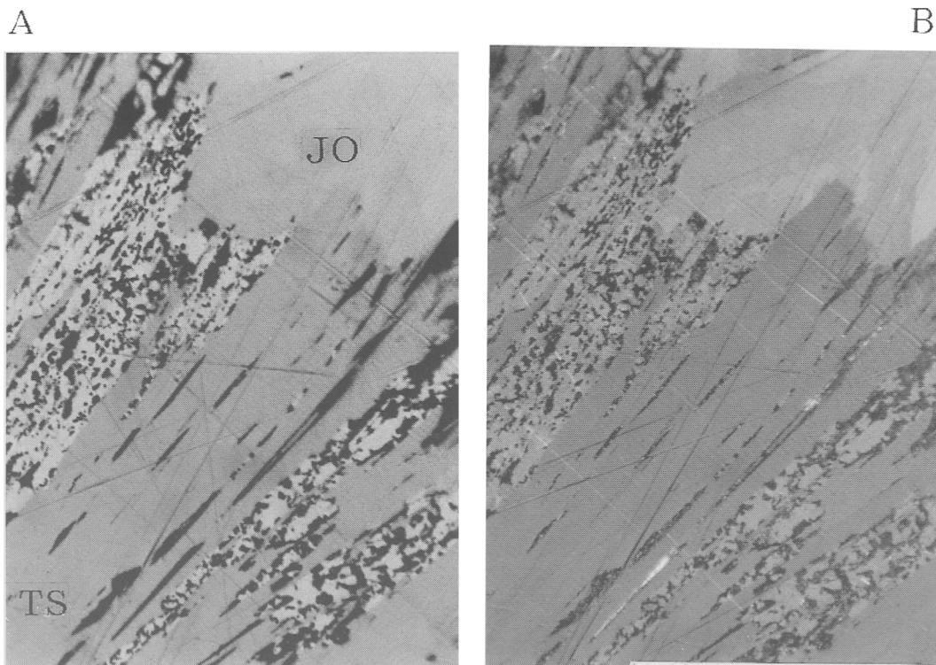
FIG. 2. Photomicrograph of tabular tsugaruite (TS) on massive jordanite (JO). (A) in plane polarised light, (B) with crossed polars; scale bar 100 \mu\text{m} . Oil immersion.
