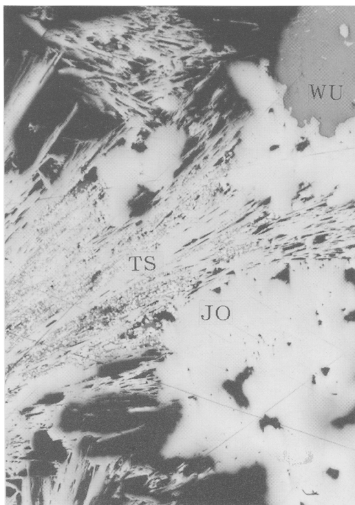
FIG. 1. Photomicrograph of tabular tsugaruite (TS) on massive jordanite (JO). (A) in plane polarised light, (B) with crossed polars; scale bar 500 \mu\text{m} .
