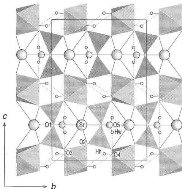
FIGURE 2. The Cmcm structure of hennomartinite at 245 °C projected along [100]. The edge-sharing, Jahn-Teller-distorted MnO_6 octahedra form rods parallel to [100], which are interconnected by Si_2O_7 groups. The interstices of the framework are occupied by Sr atoms (large spheres) and H_2O molecules (O5 = medium spheres), and by the H atoms (small spheres) of the OH groups. Dotted lines represent O \cdots H bonds between 2.0 and 2.1 Å.
