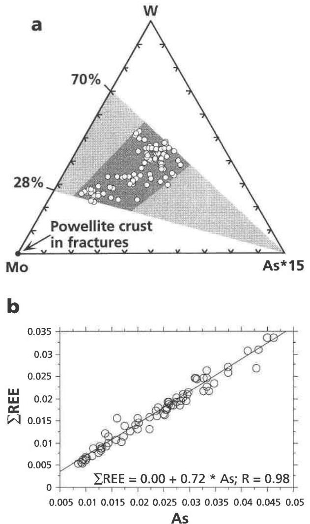
FIGURE 6. (a) Triangular plot of all EMP analyses of scheelite-powellite from Fianel (molar proportions). (b) a plot of formula proportions of \Sigma\text{REE} vs. As (normalized to four O atoms).
