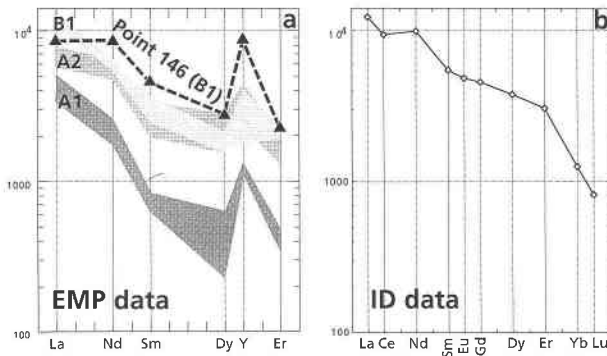
FIGURE 7. (a) Chondrite-normalized REE pattern for sample Sc2/10; data from EMP analyses (Table 3); (b) Chondrite-normalized REE pattern for scheelite-powellite grain JB311; data from ID analysis (Table 4). Chondrite data are from Taylor and McLennan (1985).
