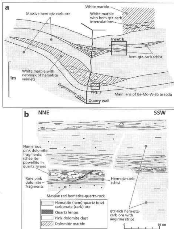
FIGURE 2. Geometry of the scheelite-powellite-bearing mineralization at Fianel, Val Ferrera (Central Alps, Switzerland).
