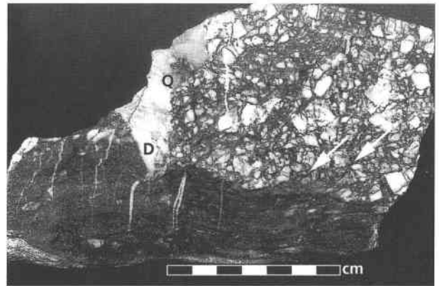
FIGURE 3. Contact between the main pink dolomite breccia and the dark embedding hematite-quartz-carbonate ore. The discordant quartz (Q) + dolomite (D) veinlets contain the Be-, Mo-, W-, and Sb-minerals. Shear bands penetrating the breccia are indicated by arrows.
