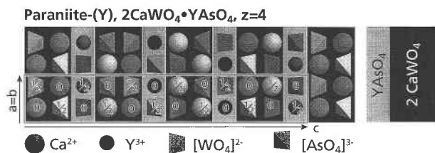
FIGURE 1. Structure of paraniite-(Y) after Demartin et al. (1992). The structure consists of a regular stacking of two scheelite layers (black) and one \text{YAsO}_4 layer (gray). The vertical displacements along the a = b axis are indicated ( \frac{1}{2} or 0).
