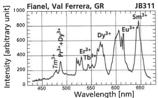
FIGURE 8. Thermal X-ray luminescence spectrum of scheelite-powellite grain JB311. Analytical conditions: 250 °C, 30 kV, and 60 μA.
