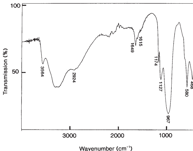
FIG. 2. The infrared spectrum of ercittite
