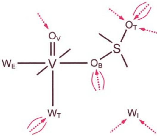
FIG. 7. Summary of the possible hydrogen-bond linkages in vanadium sulfate hydrates; V and S denote cation sites, O B denotes the anion bridging between the (V \phi_6 ) and (SO 4 ) polyhedra, O V is the vanadyl O-atom, O T is a terminal O-atom, W E is an equatorial (H 2 O) group, W T is a trans (H 2 O) group, W I is an isolated (H 2 O) group. Broken red lines denote required hydrogen-bonds; broken red lines in parentheses indicate possible hydrogen-bonds.
