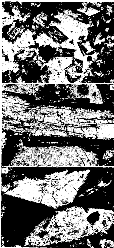
FIG. 1. a: Killalaité crystals in a vein of calcite. The squarish crystal (right middle) is \frac{1}{2} mm. across. b: A longitudinal section of killalaité showing two cleavages, the length is close to 2 mm. c: A section nearly parallel to (010) showing the (100) cleavage trace and the penetration twinning, crystal size as in a. All three photomicrographs taken under partially crossed nicols.
