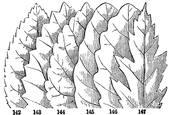
From left to right: Serrate, Dentate, Crenate, Way, Sinuate, Incised
