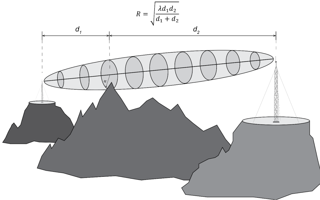
FIGURE 3-1. Effective Ellipsoid Shape
