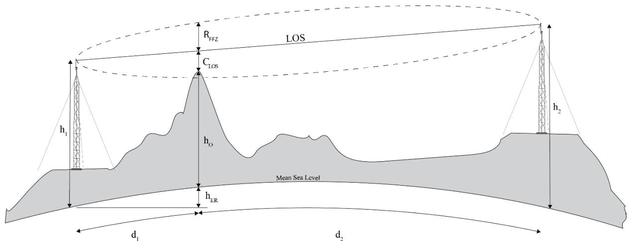
FIGURE 3-2. Path Profile Traversing Uneven Terrain with Knife-Edge Obstruction
