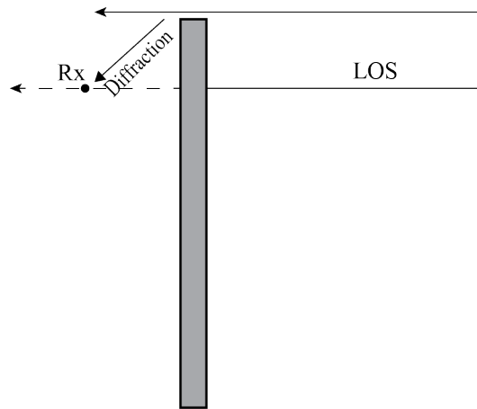
FIGURE 1-3. Totally Obstructed LOS
