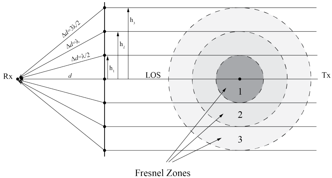
FIGURE 2-1. Fresnel Zones
