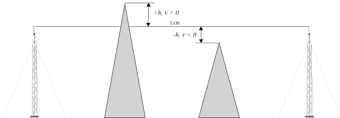
FIGURE 5-1. Diffraction Parameter
