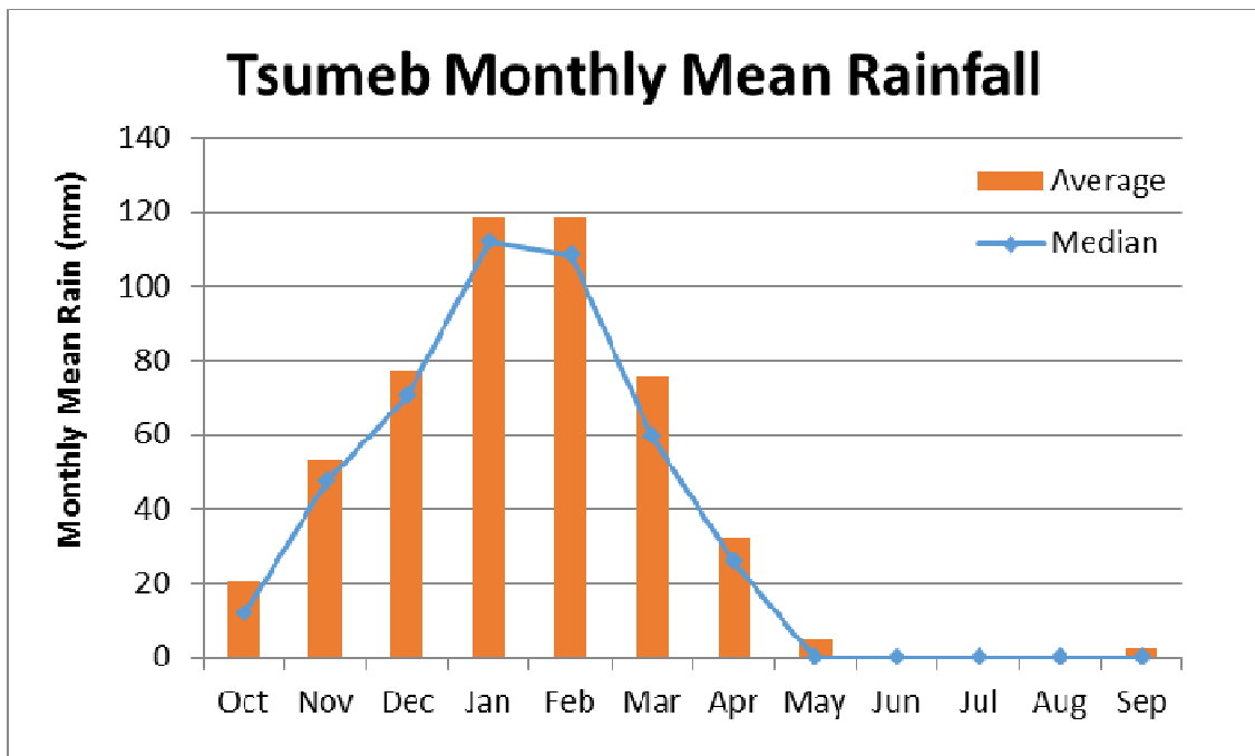
FIGURE 4: TSUMEB MONTHLY MEAN RAINFALL DISTRIBUTION
