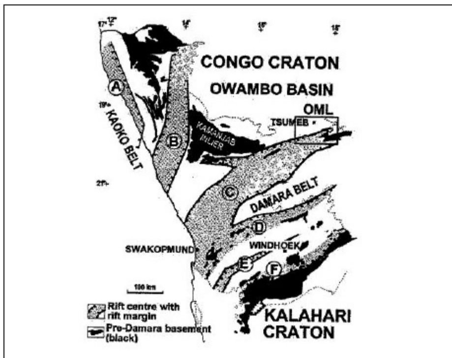
Figure 2.4: Location of the Otavi Mountain Land (OML), the Owambo Basin and the presumed location of the continental rift structures during the rifting stage of the Damara and Kaoko Belts (from Porada 1989). A = Kaoko Rift, B =Sesfontein, C = Northern Rift, D = Central Rift, E = Khomas Rift, F =Southern Rift. Note that the southern and eastern limits of the Owambo Basin are defined by the Northern boundaries of the Kamanjab inlier and the Northern Rift (C) as well as the eastern margin of the Sesfontein Rift (B). Modified after Kamona and Gunzel, (2006)
