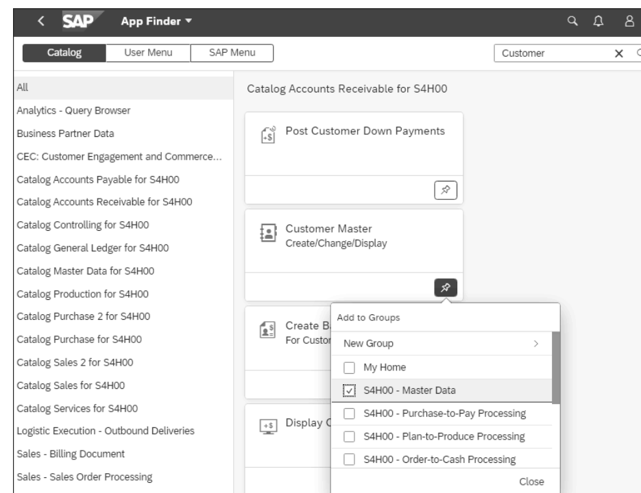
Figure 6.25 Adding the App to a Group
