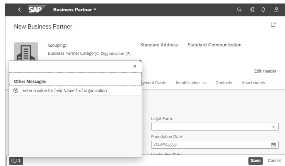
Figure 6.18 Footer Toolbar with Message Icon at the Bottom Left
