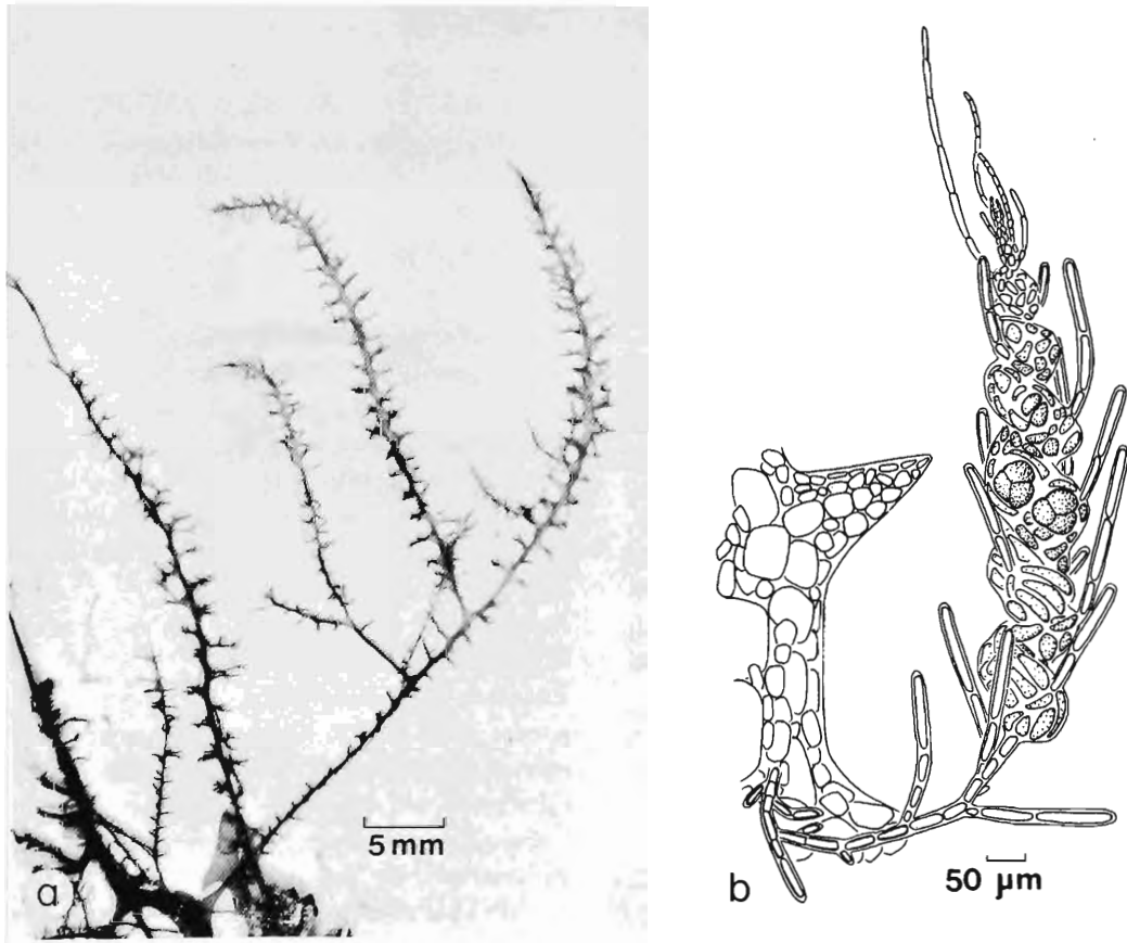
FIGURE 106.— Wrihtiella blodgettii (JN-7046): a , portion of the thallus showing branches with numerous spur branchlets; b , portion of main axis with a spiral tetrasporangial stichidia.
