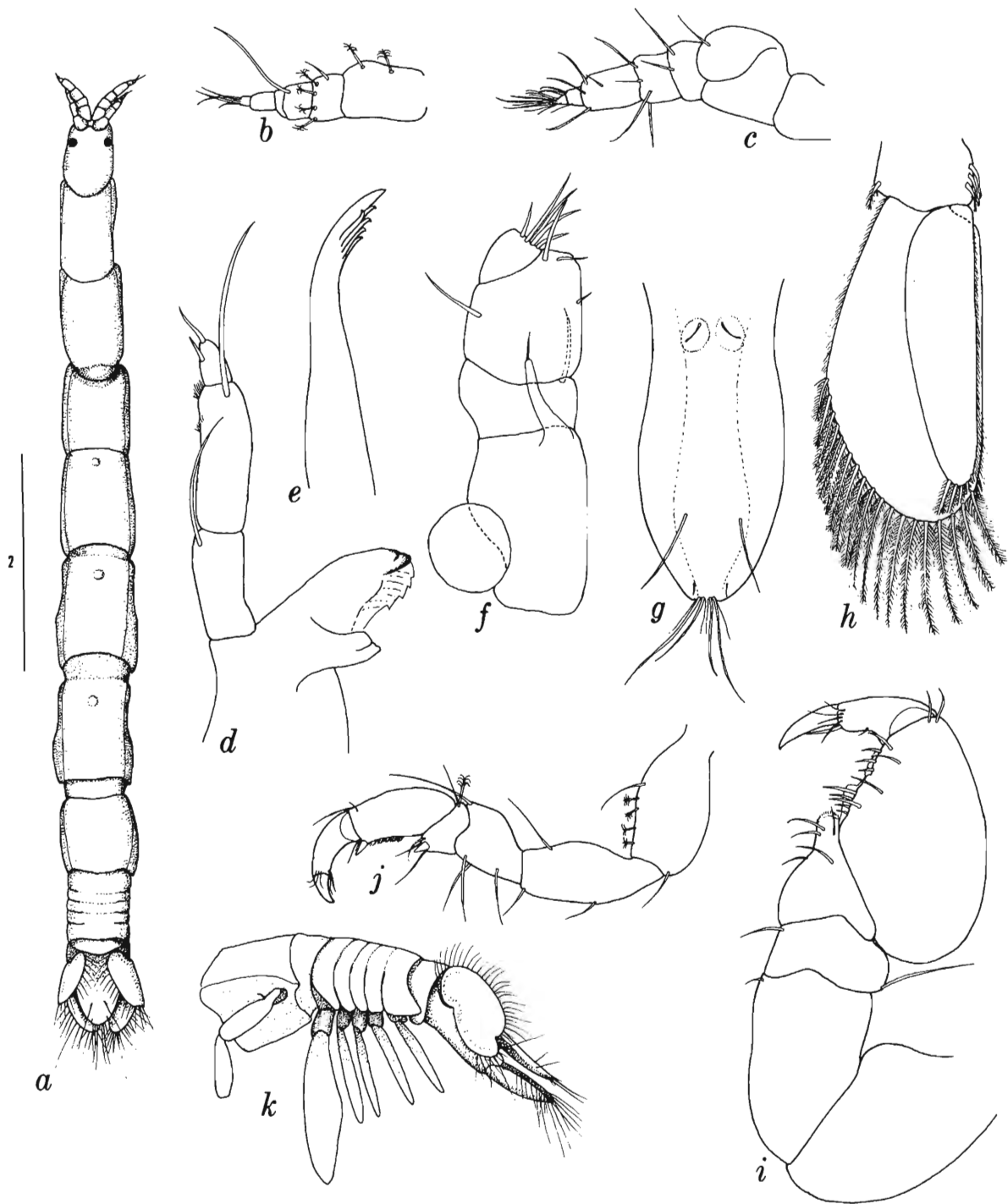
FIGURE 141.— Apantura geminsula , new species, holotype, ♀: a , complete specimen; b , antennule; c , antenna; d , mandible; e , maxilla; f , maxilliped; g , telson; h , pleopod 1; i , pereopod 1; j , pereopod 7; k , pleon in lateral view.
