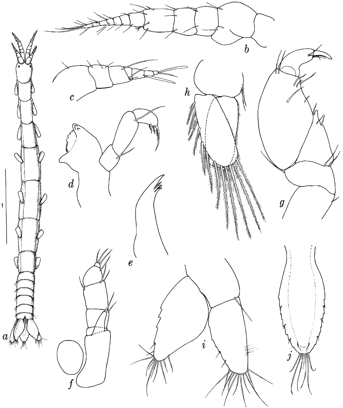
FIGURE 146.— Belizanthura imswe , new species, holotype, ♀: a , complete specimen; b , antenna; c , antennule; d , mandible; e , maxilla; f , maxilliped; g , pereopod 1; h , pleopod 1; i , uropod; j , telson.
