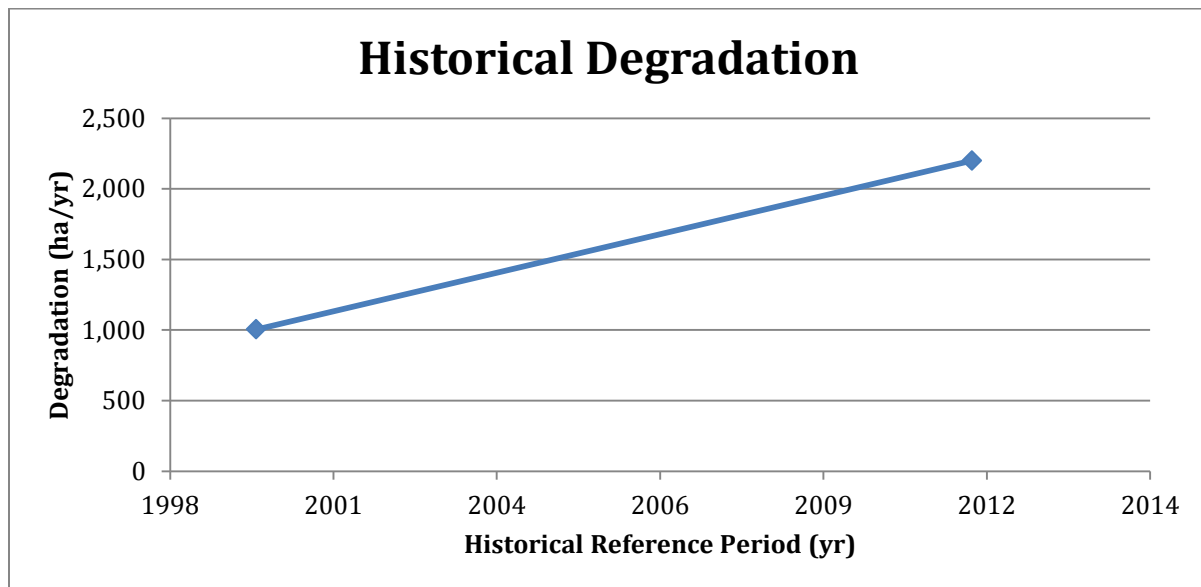
Figure 22. Historical degradation rates in reference region (ha/yr) versus time (yr) for each consecutive pair of images in the historical reference period.
