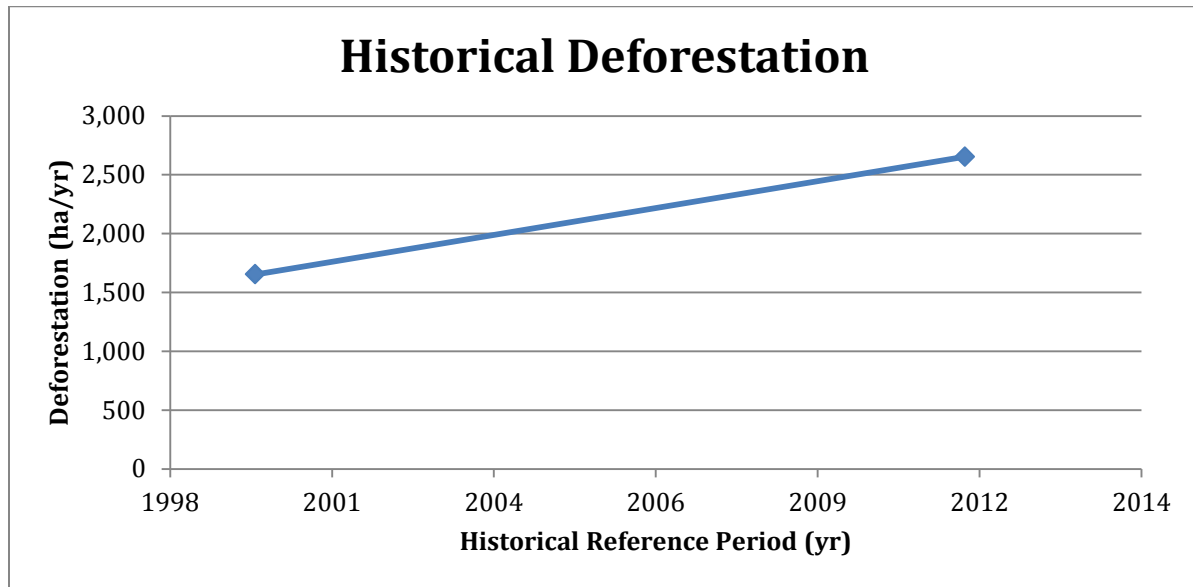
Figure 21. Historical deforestation rates in reference region (ha/yr) versus time (yr) for each consecutive pair of images in the historical reference period.
