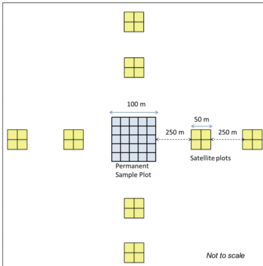
Figure 20. Map of cluster plots relative to permanent plots in RAINFOR configuration.
