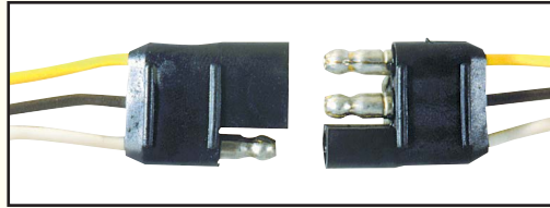
TC30 3-Pole Molded Trailer Connector • 18 gauge pigtails for boats, trailers, etc. • Plug and receptacle are not sold separately
