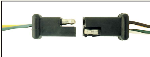
TC46 Universal 4-Pole Square Type Connector • 12" leads
