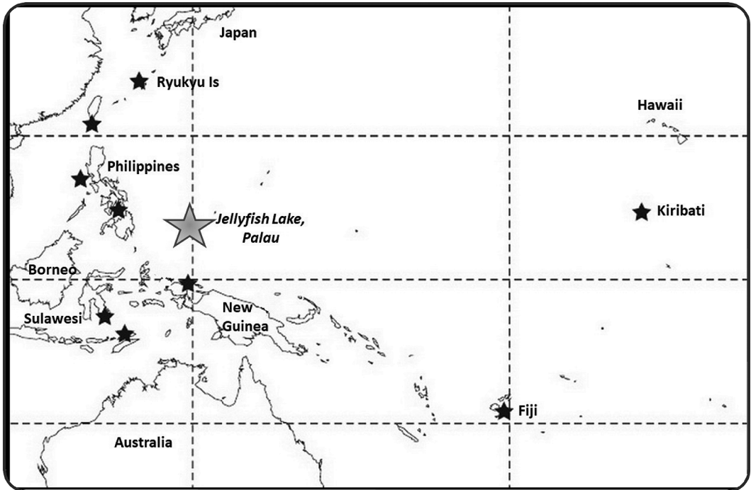
FIGURE 8. Central and Western Pacific showing the distribution of Phanerophthalmus luteus (black stars) and the location of Jellyfish Lake, Palau (large gray star). Modified from distribution map for P. luteus in Austin, Gosliner, and Malaquias (2018, fig. 23).
