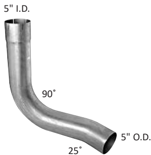
68183 Replaces KENWORTH Part No. 180B-10742-L Left Side Elbow with Offset
