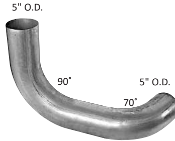
38607 Replaces INTERNATIONAL / NAVISTAR Part No. 503-845-C1 89" Cab
