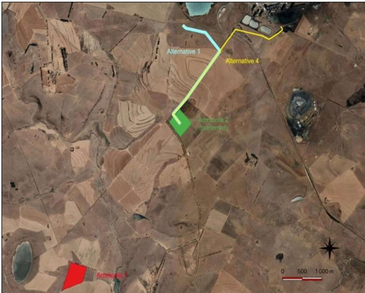
Figure 7: Pipeline alternatives for Ammonia 2.
